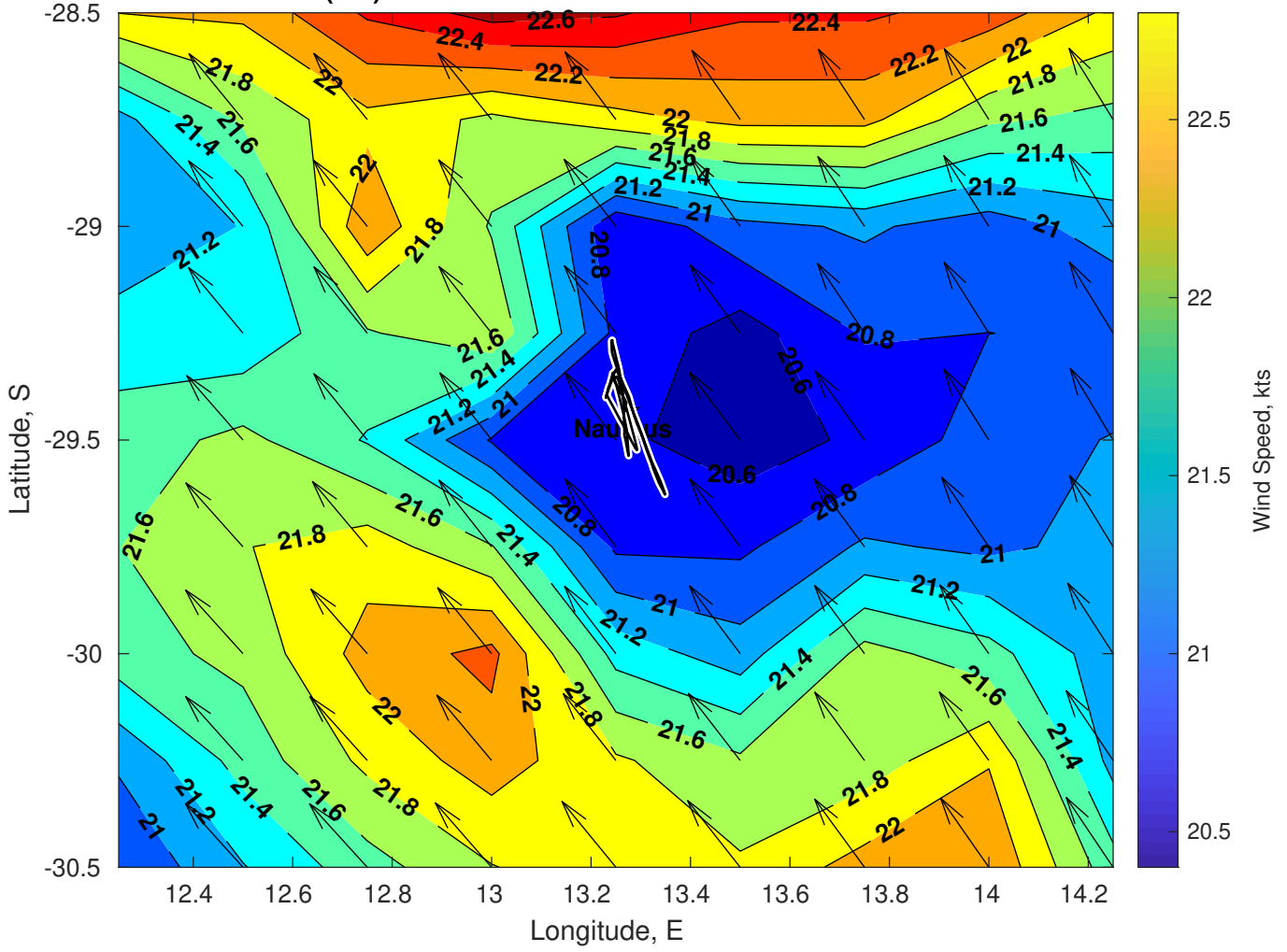
Winds (kts) for Nautilus at 25-Feb-2025 09:00:00
