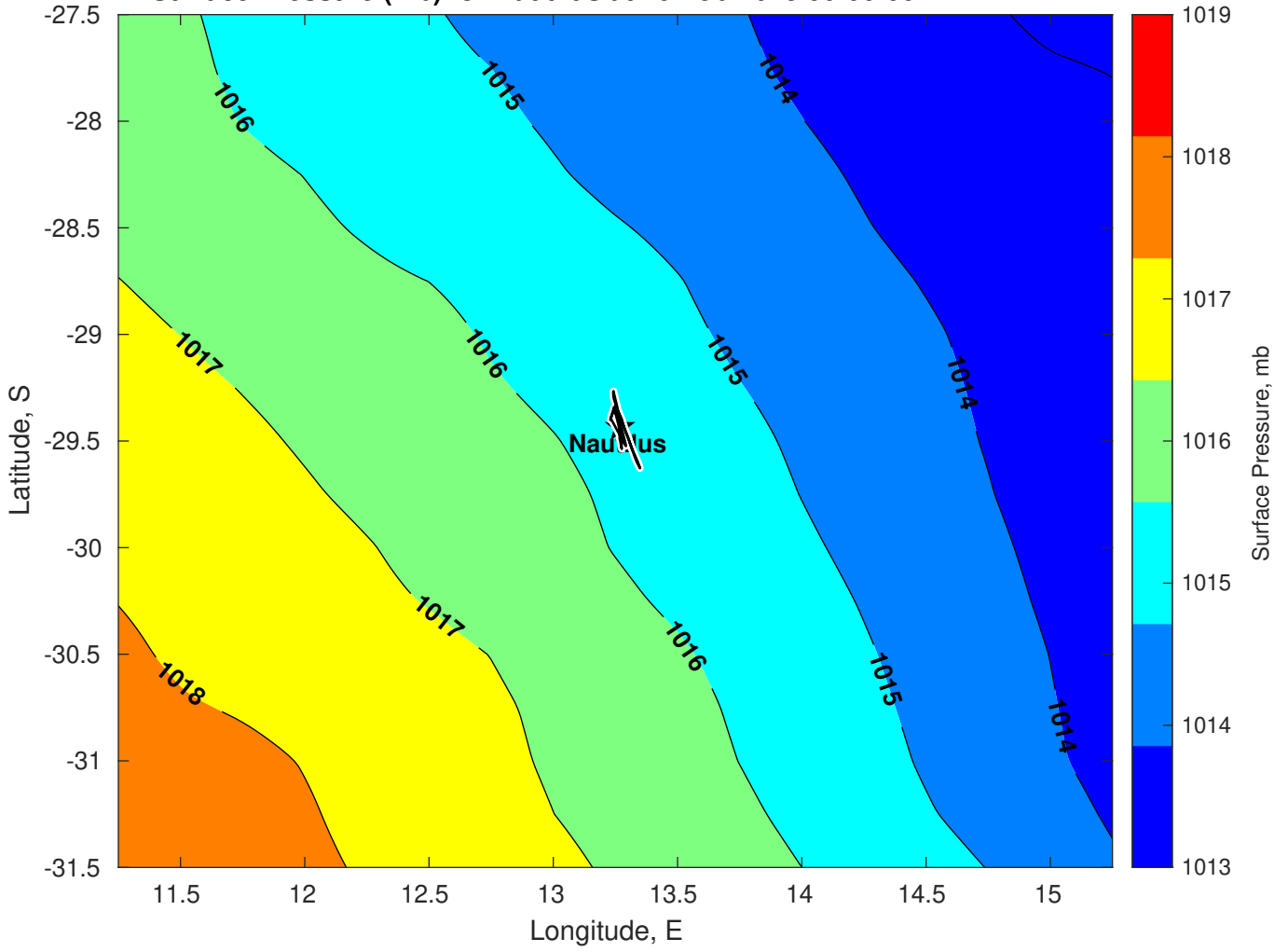
Surface Pressure (mb) for Nautilus at 26-Feb-2025 00:00:00
