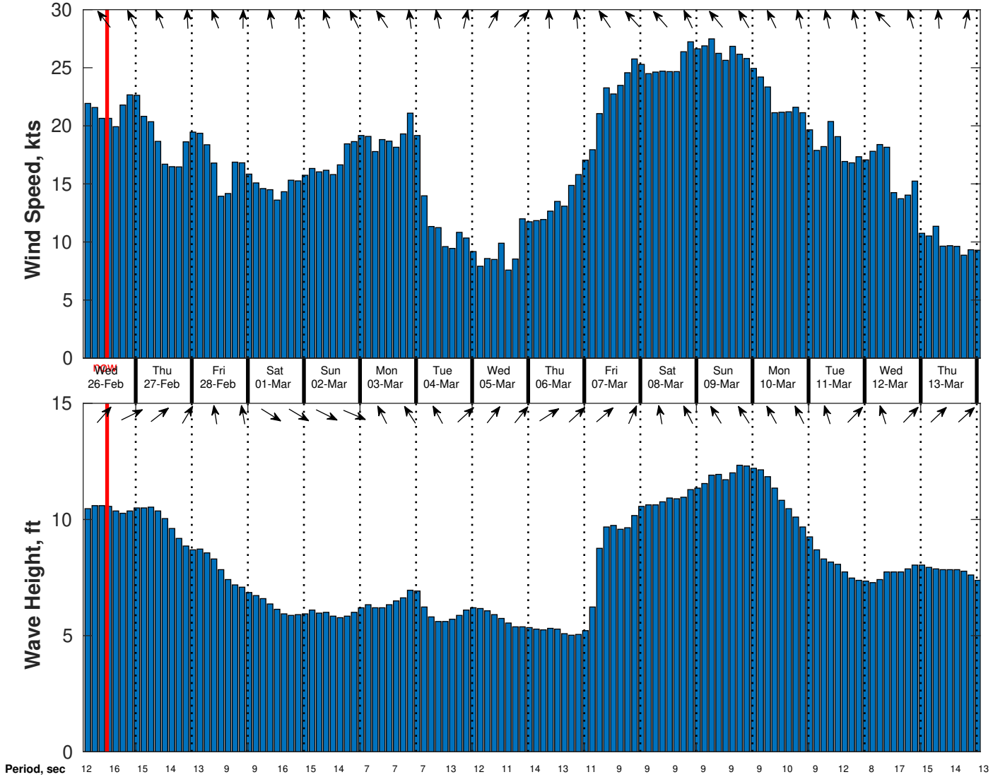
Wind & Wave Forecast for Nautilus from 25-Feb-2025 02:00:00 to 13-Mar-2025 02:00:00
