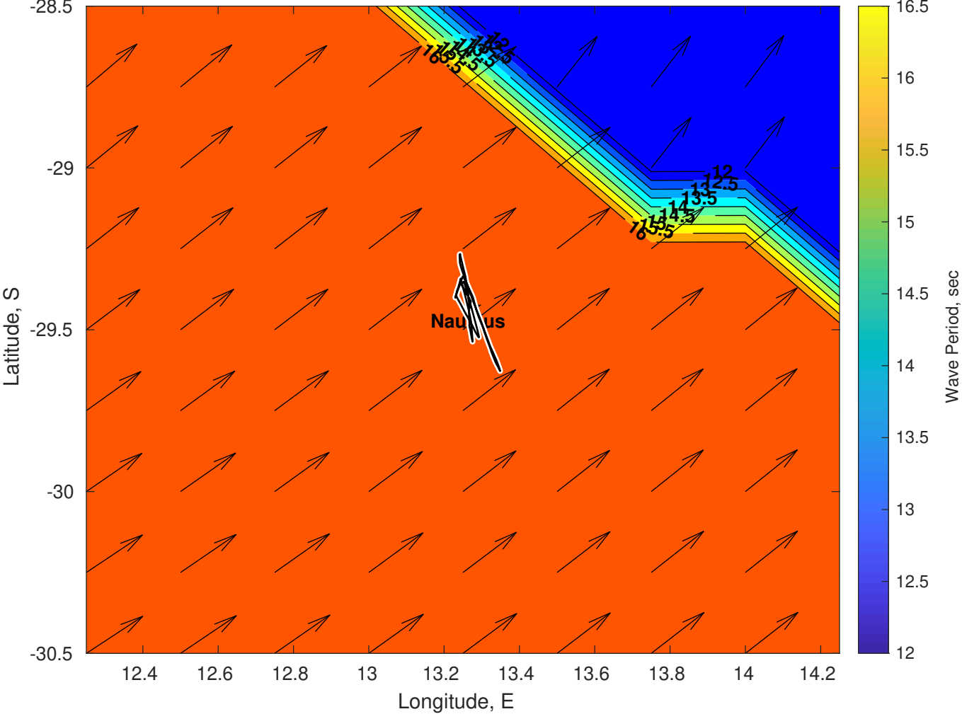
Wave Period (sec) for Nautilus at 25-Feb-2025 09:00:00
