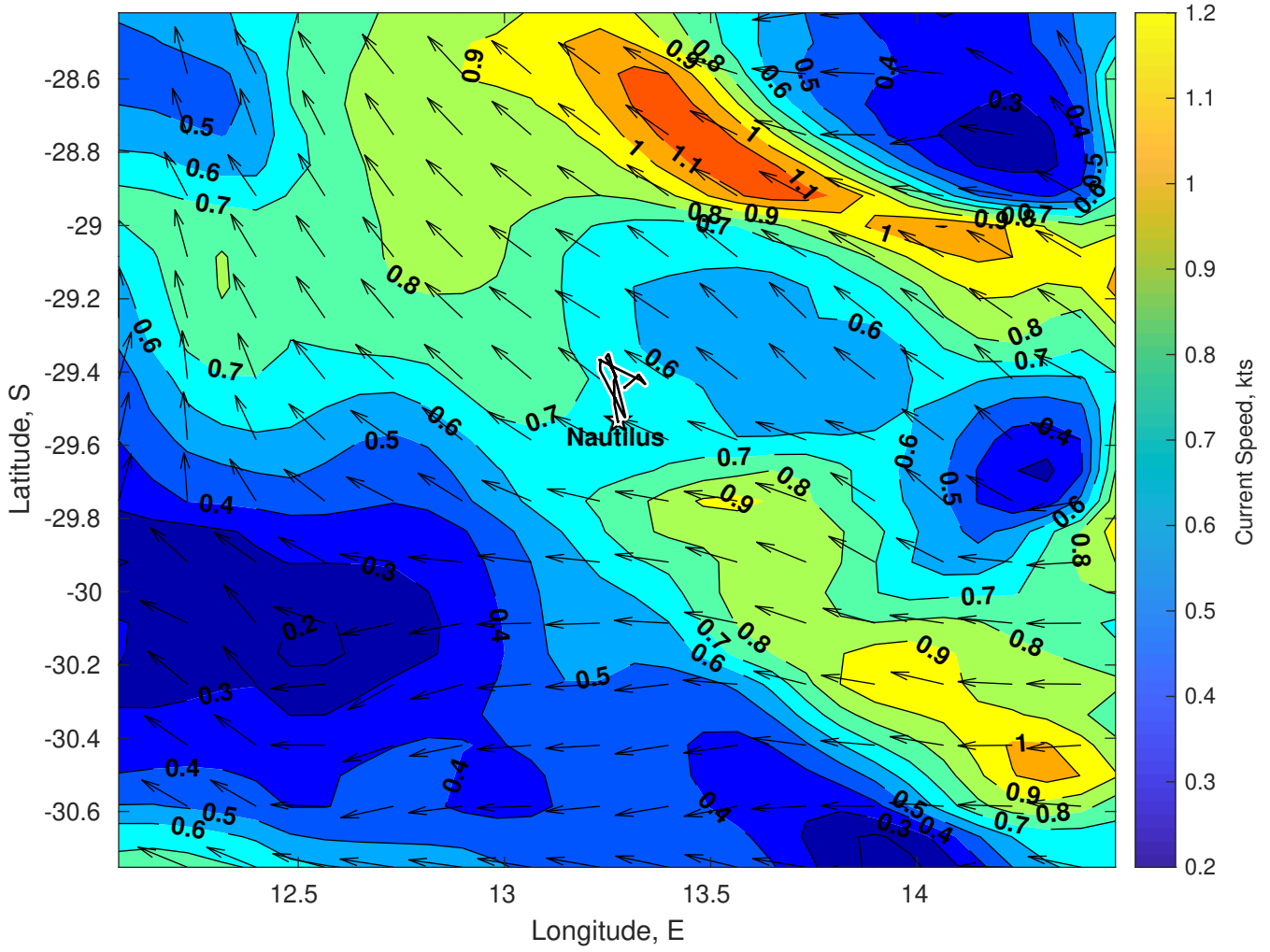
Surface Currents for Nautilus at 24-Feb-2025 00:00:00
