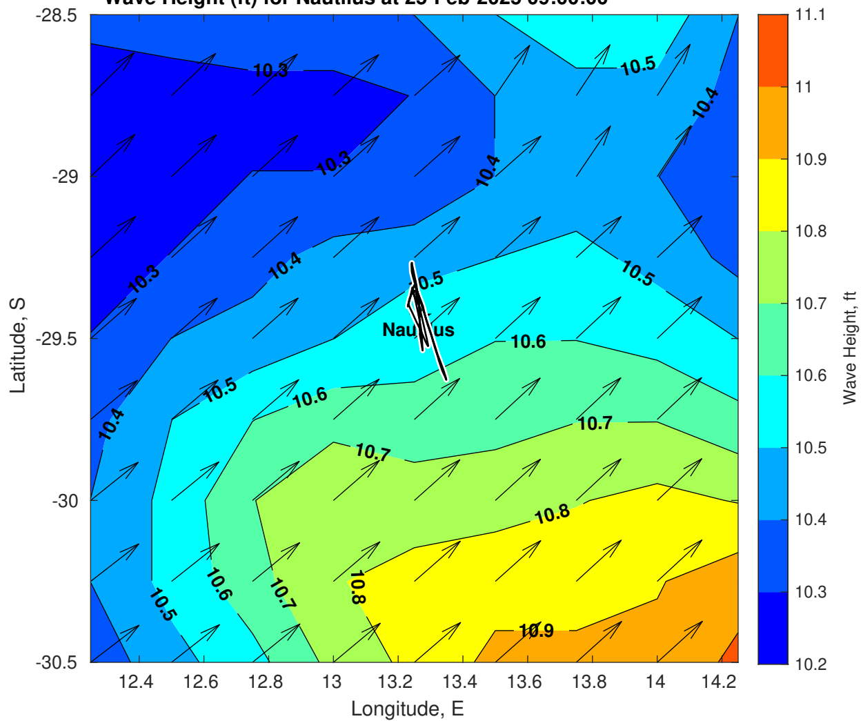
Wave Height (ft) for Nautilus at 25-Feb-2025 09:00:00
