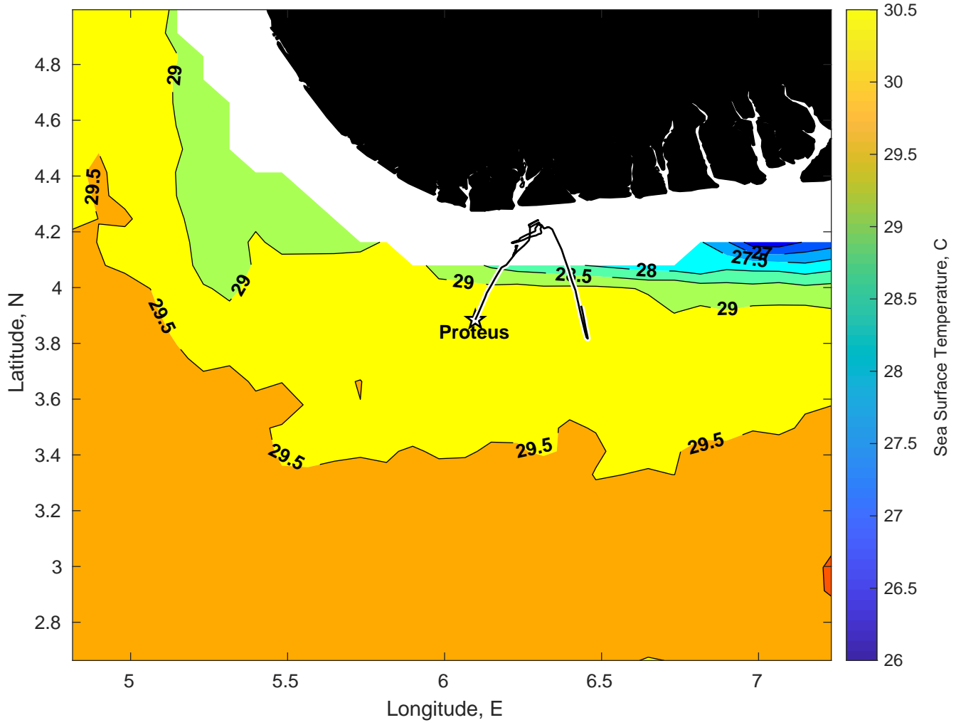
SST for Proteus at 24-Feb-2025 00:00:00
