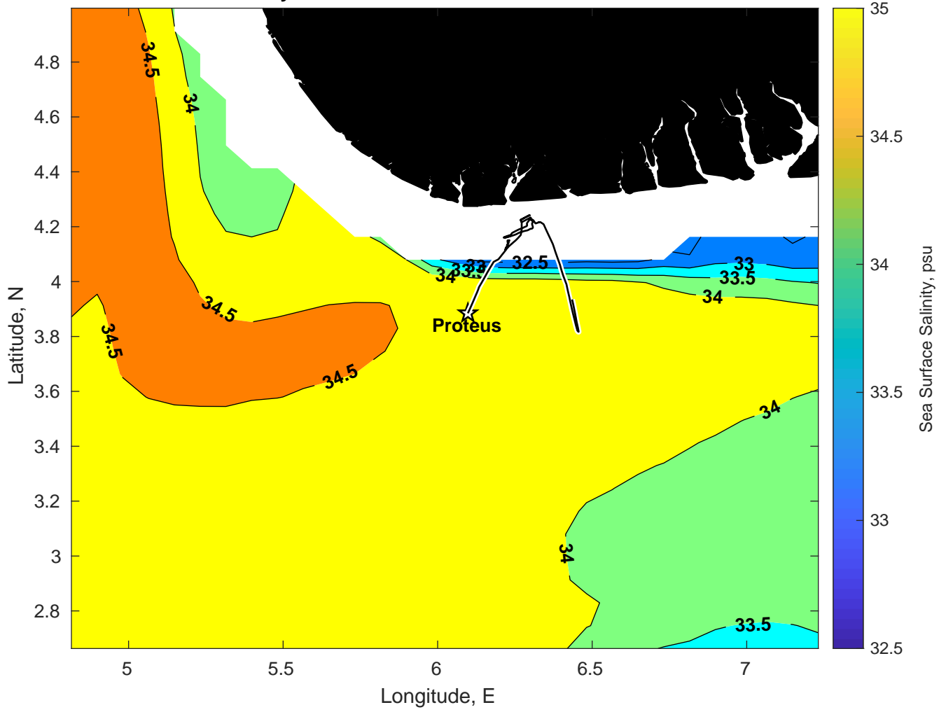
Surface Salinity for Proteus at 24-Feb-2025 00:00:00
