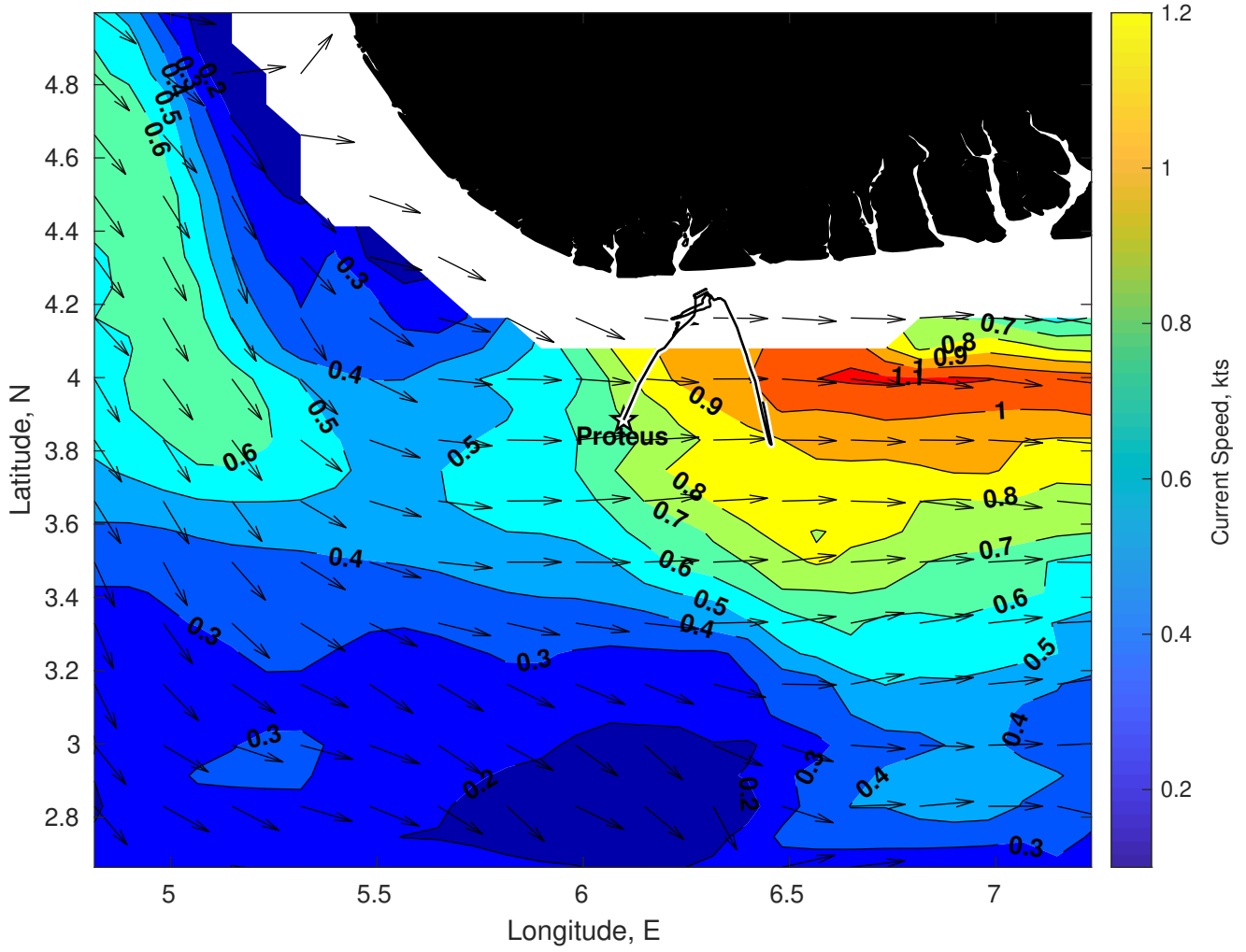
Surface Currents for Proteus at 24-Feb-2025 00:00:00
