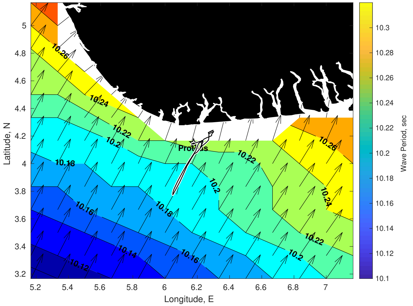
Wave Period (sec) for Proteus at 25-Feb-2025 09:00:00
