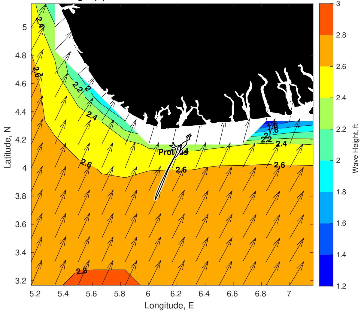
Wave Height (ft) for Proteus at 25-Feb-2025 09:00:00
