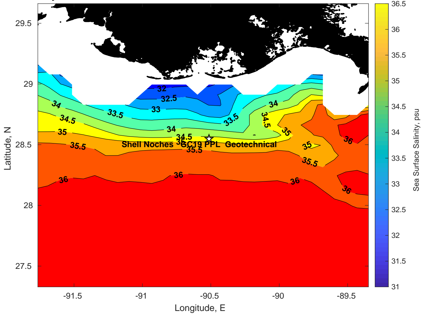
Surface Salinity for Shell Noches GC19 PPL Geotechnical at 24-Feb-2025 00:00:00
