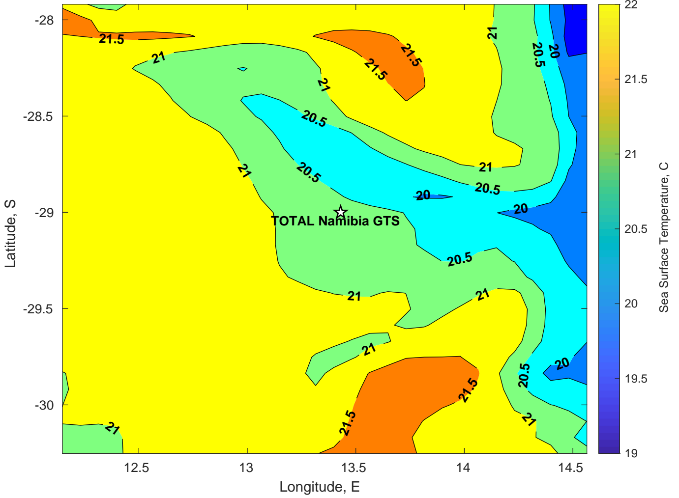
SST for TOTAL Namibia GTS at 24-Feb-2025 00:00:00
