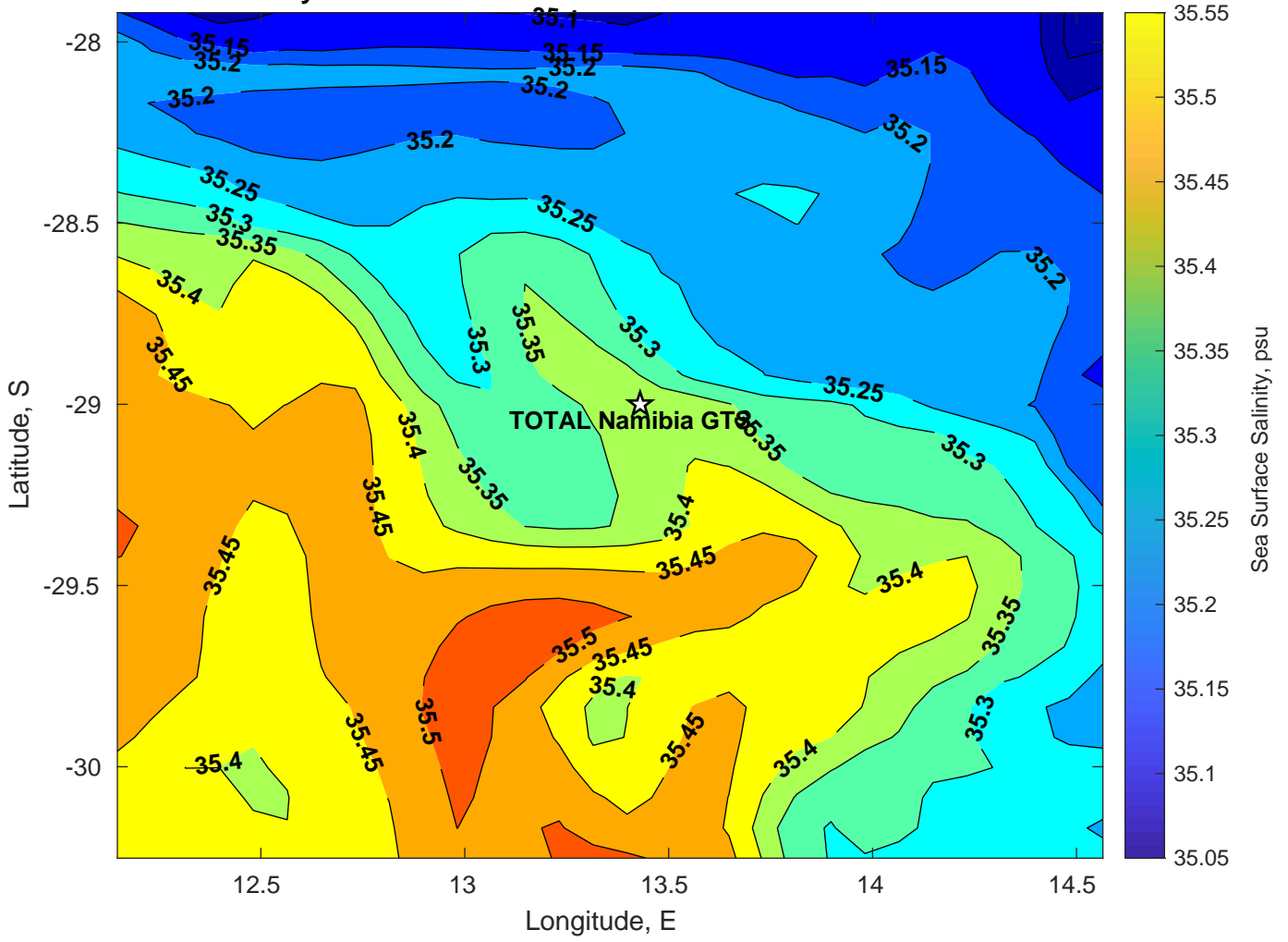
Surface Salinity for TOTAL Namibia GTS at 24-Feb-2025 00:00:00
