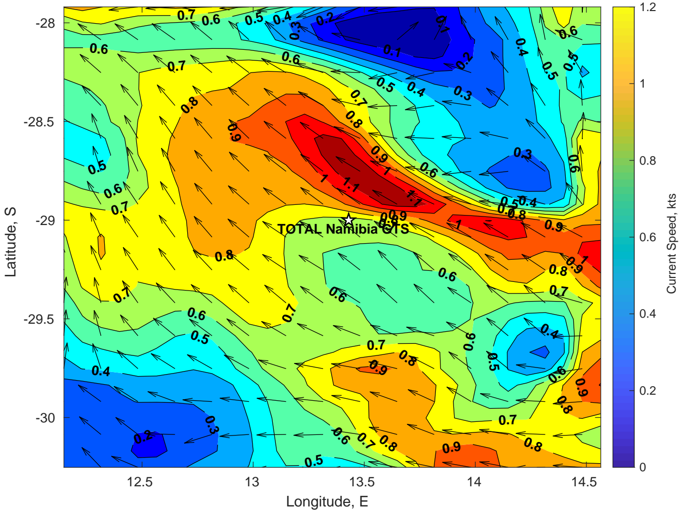
Surface Currents for TOTAL Namibia GTS at 24-Feb-2025 00:00:00
