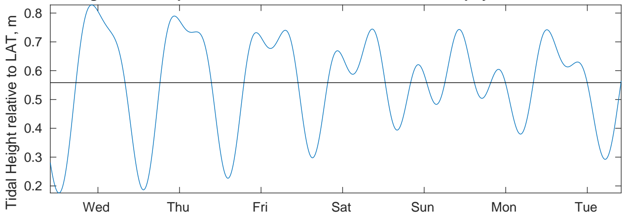
Tidal Currents and Heights for Tampnet P2378 South Texas Cable Route Geophysical at 20250225
