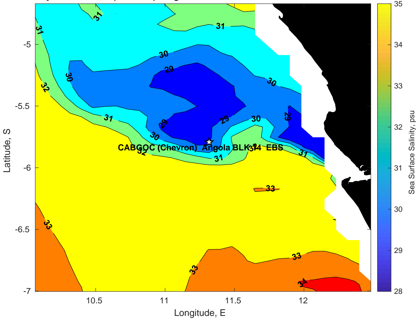
Surface Salinity for CABGOC (Chevron) Angola BLK 14 EBS at 25-Feb-2025 00:00:00
