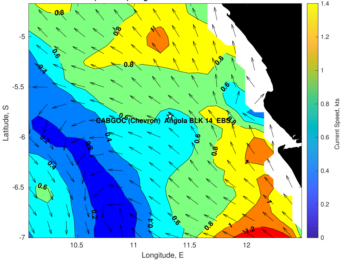
Surface Currents for CABGOC (Chevron) Angola BLK 14 EBS at 25-Feb-2025 00:00:00
