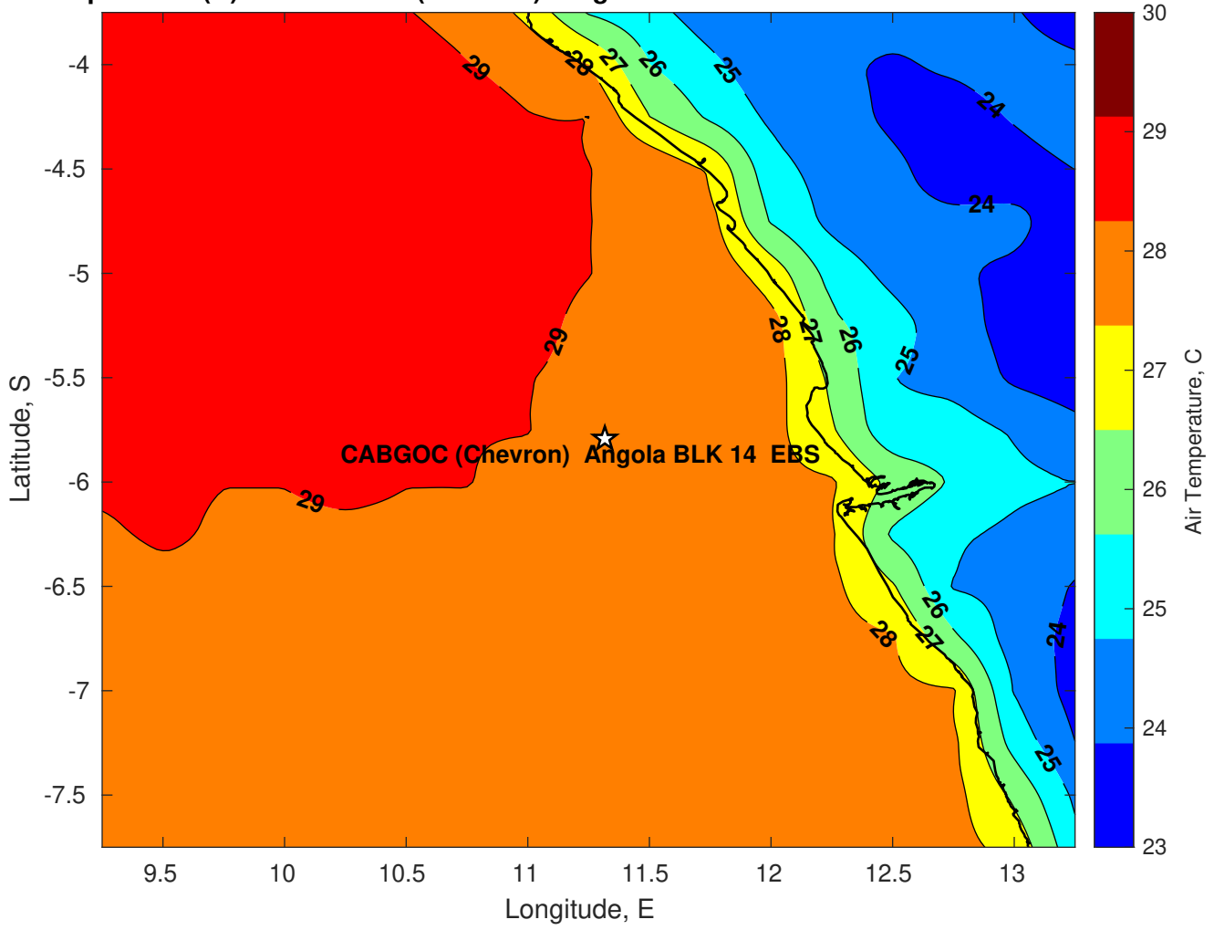
Air Temperature (C) for CABGOC (Chevron) Angola BLK 14 EBS at 26-Feb-2025
