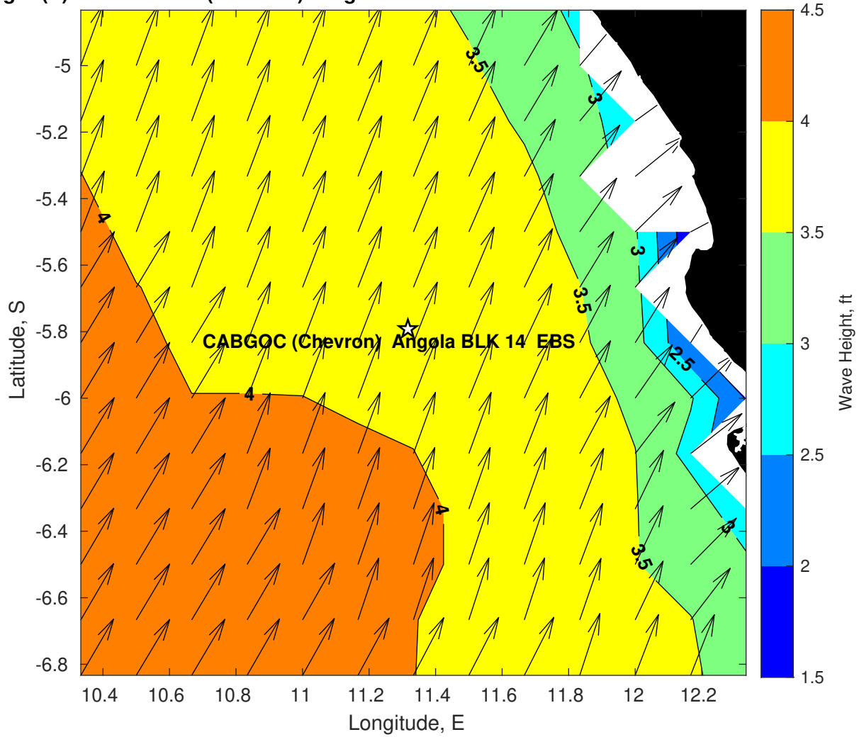
Wave Height (ft) for CABGOC (Chevron) Angola BLK 14 EBS at 26-Feb-2025 09:00:00
