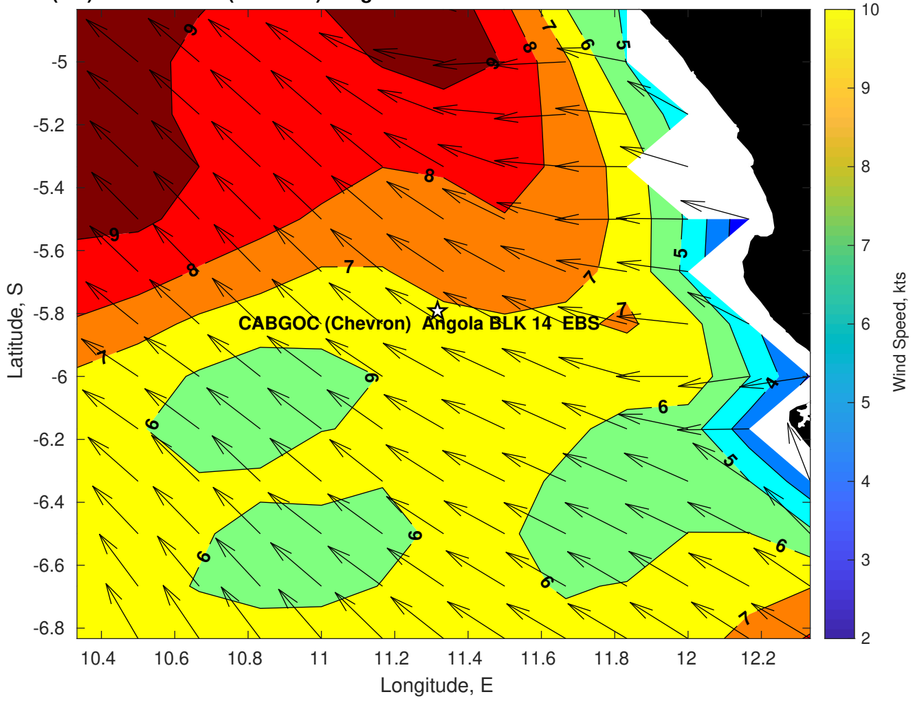
Winds (kts) for CABGOC (Chevron) Angola BLK 14 EBS at 26-Feb-2025 09:00:00
