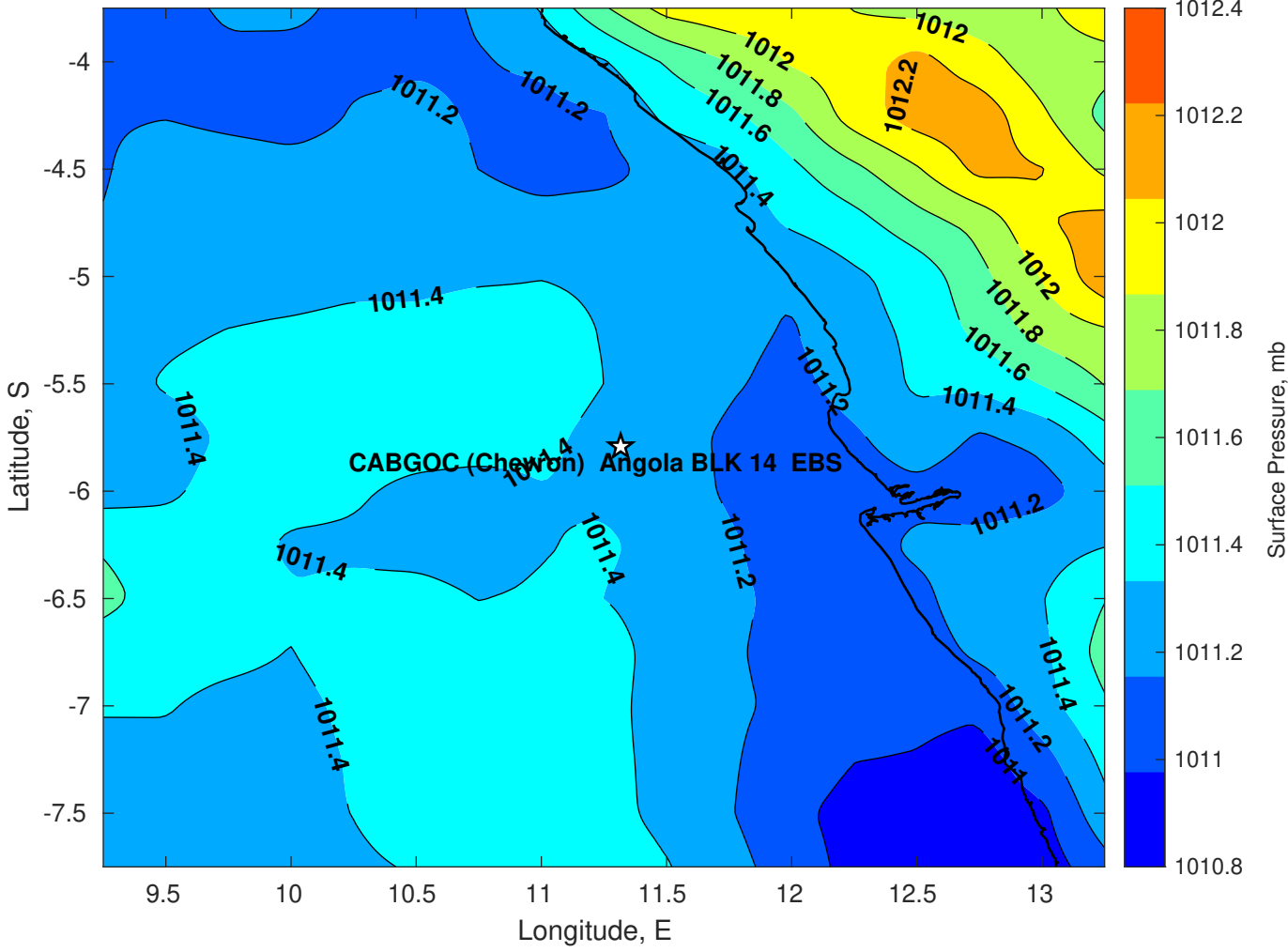
Surface Pressure (mb) for CABGOC (Chevron) Angola BLK 14 EBS at 26-Feb-2025 00:00:00
