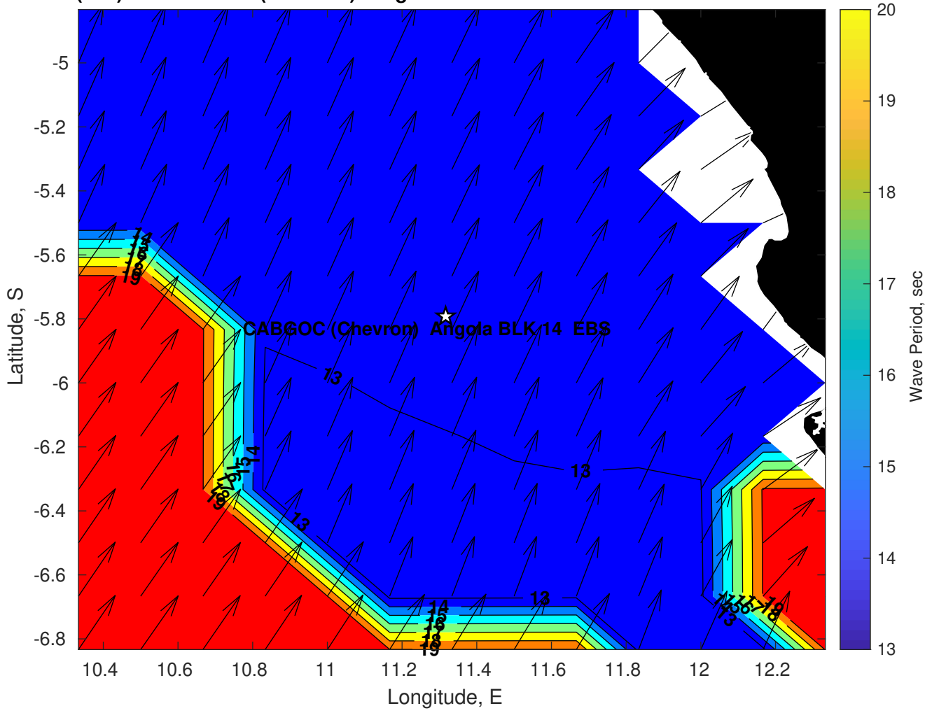
Wave Period (sec) for CABGOC (Chevron) Angola BLK 14 EBS at 26-Feb-2025 09:00:00
