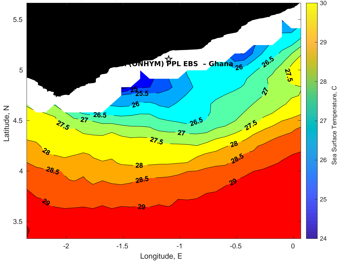
SST for CSA (ONHYM) PPL EBS - Ghana at 25-Feb-2025 00:00:00
