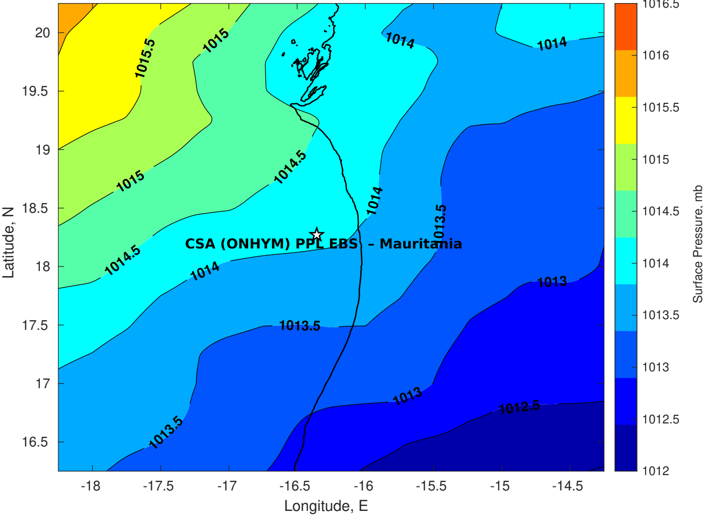
Surface Pressure (mb) for CSA (ONHYM) PPL EBS - Mauritania at 28-Feb-2025 00:00:00
