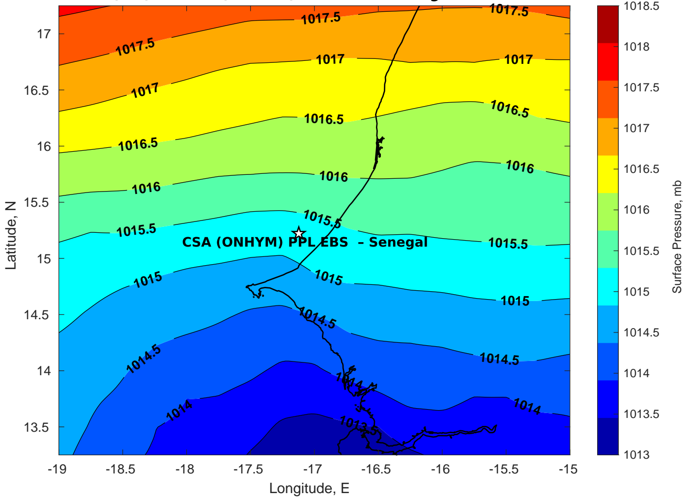
Surface Pressure (mb) for CSA (ONHYM) PPL EBS - Senegal at 26-Feb-2025 00:00:00
