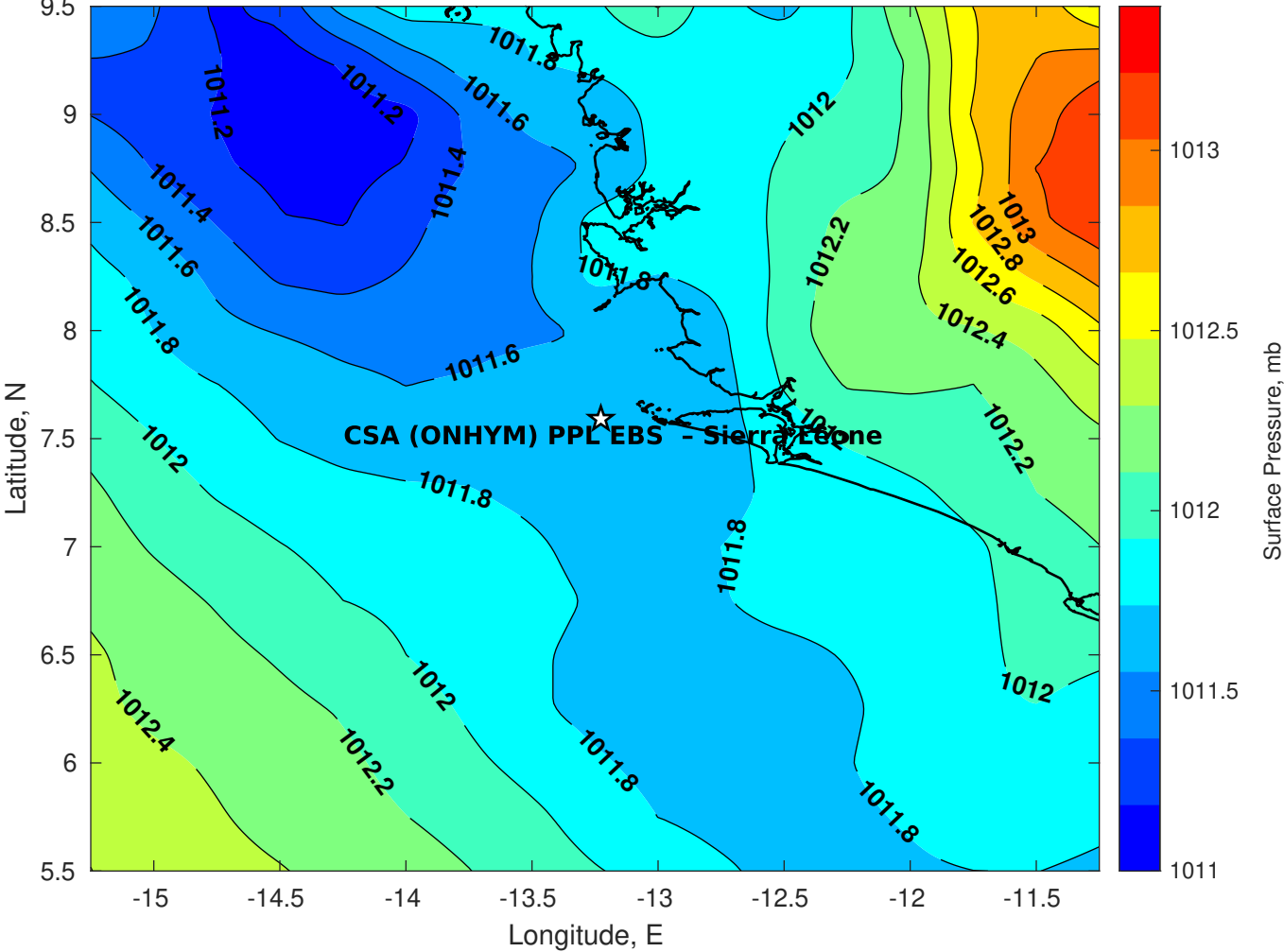
Surface Pressure (mb) for CSA (ONHYM) PPL EBS - Sierra Leone at 27-Feb-2025 00:00:00
