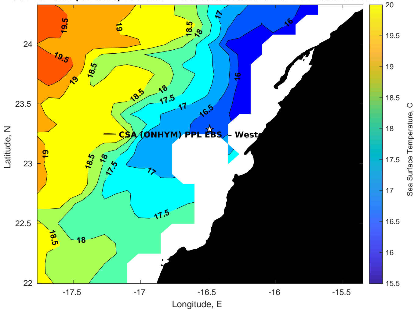
SST for CSA (ONHYM) PPL EBS - Western Sahara at 25-Feb-2025 00:00:00
