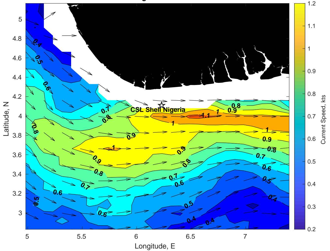
Surface Currents for CSL Shell Nigeria at 25-Feb-2025 00:00:00
