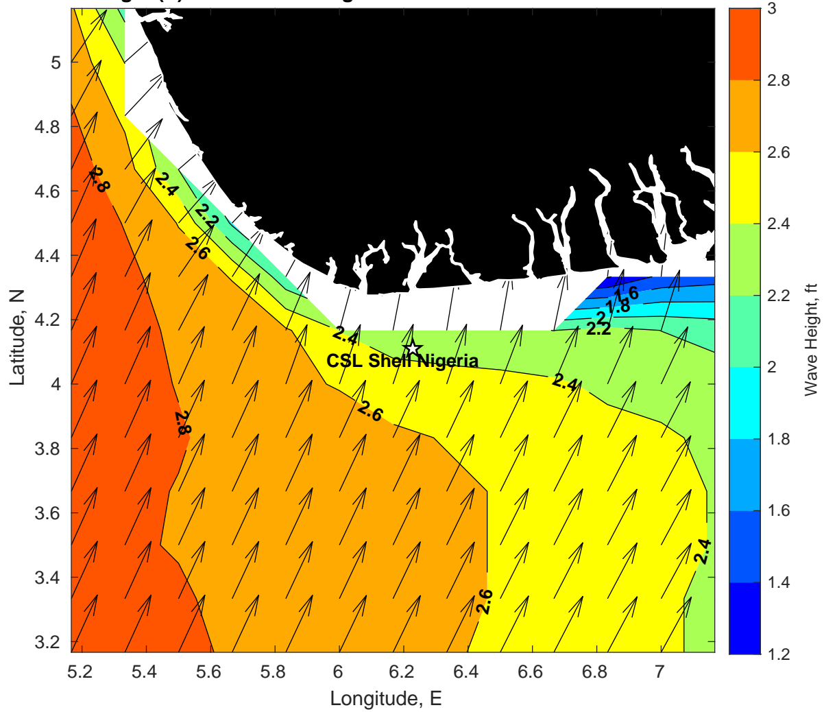
Wave Height (ft) for CSL Shell Nigeria at 26-Feb-2025 09:00:00
