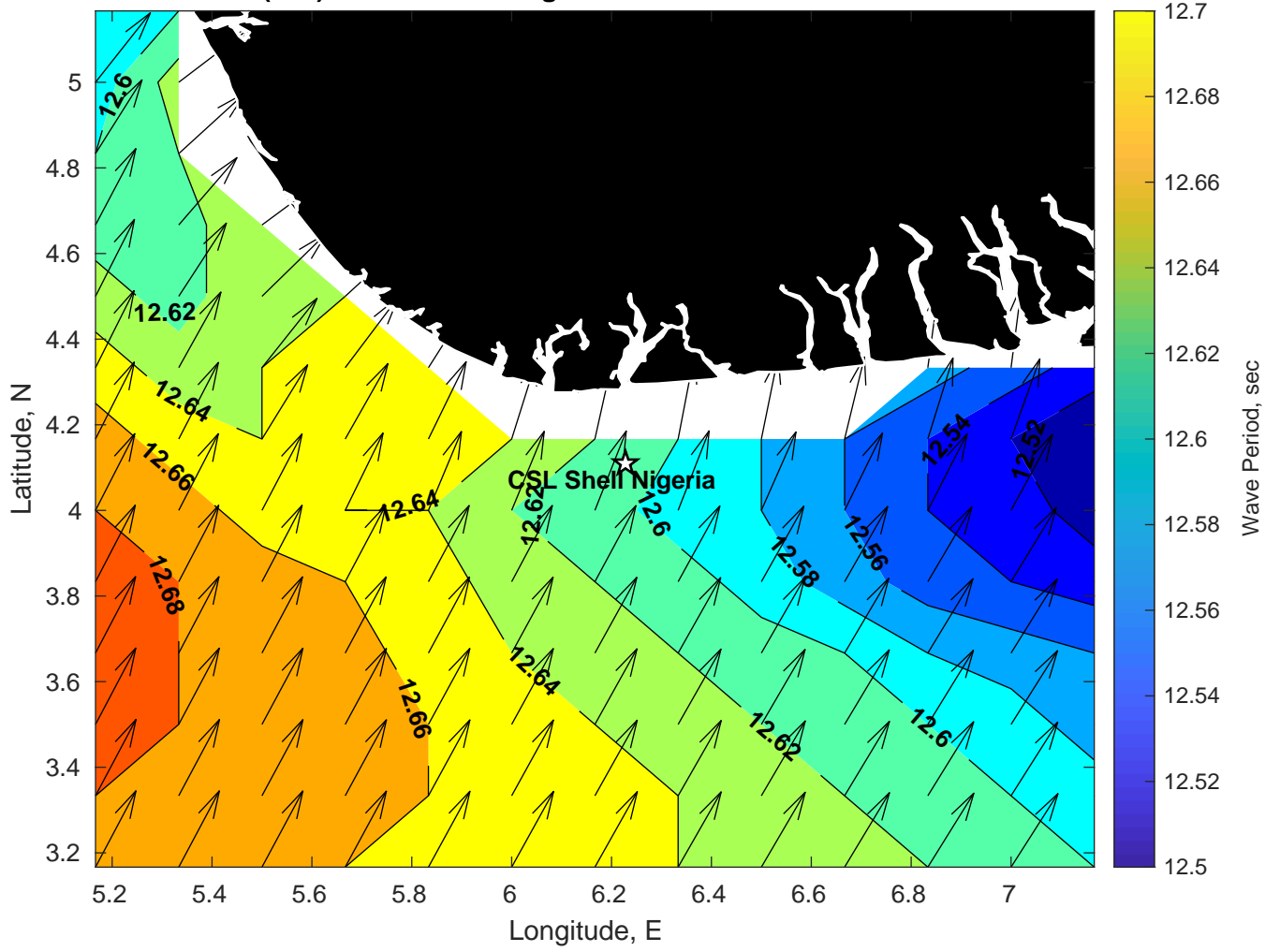
Wave Period (sec) for CSL Shell Nigeria at 26-Feb-2025 09:00:00
