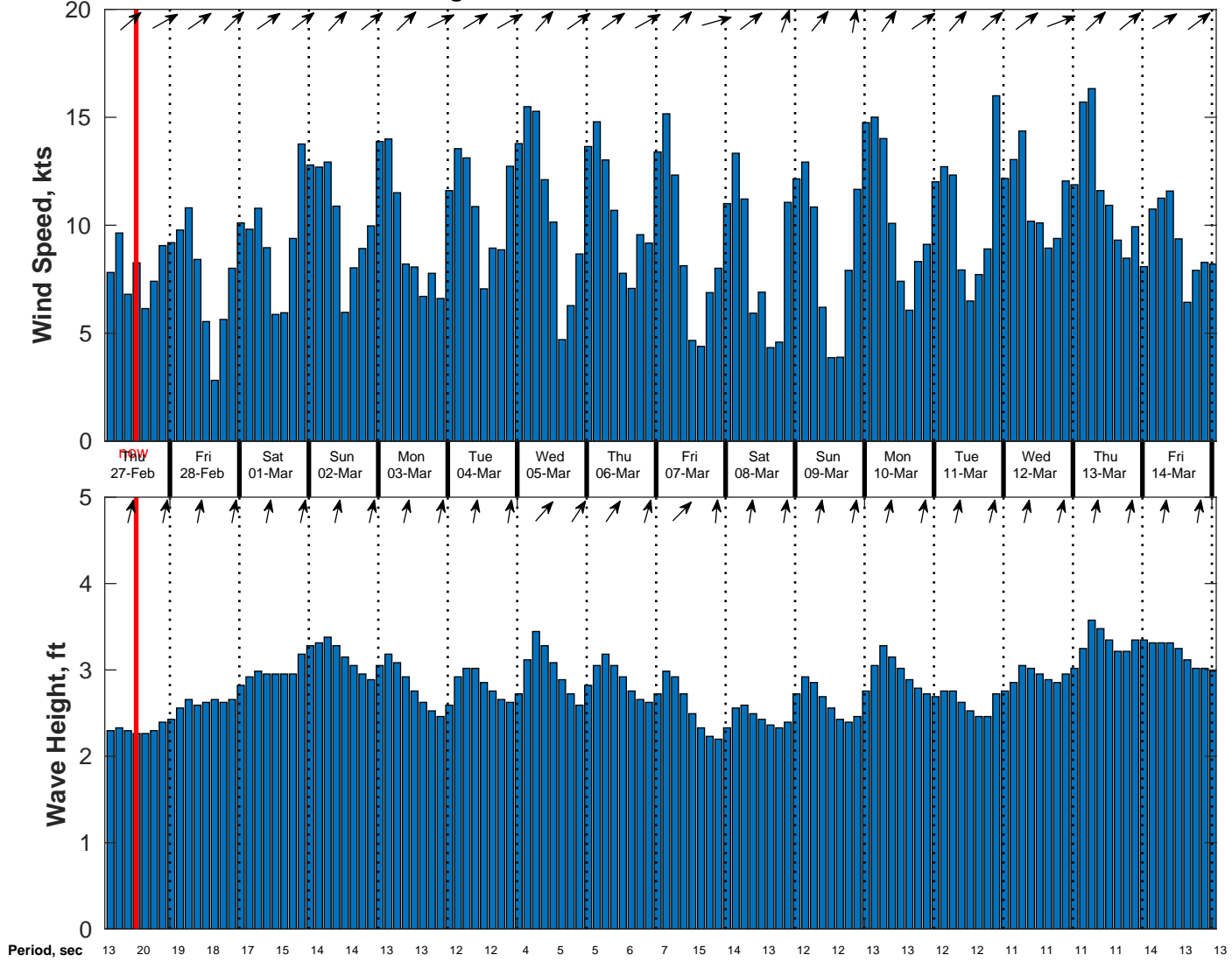
Wind & Wave Forecast for CSL Shell Nigeria from 26-Feb-2025 02:00:00 to 14-Mar-2025 02:00:00
