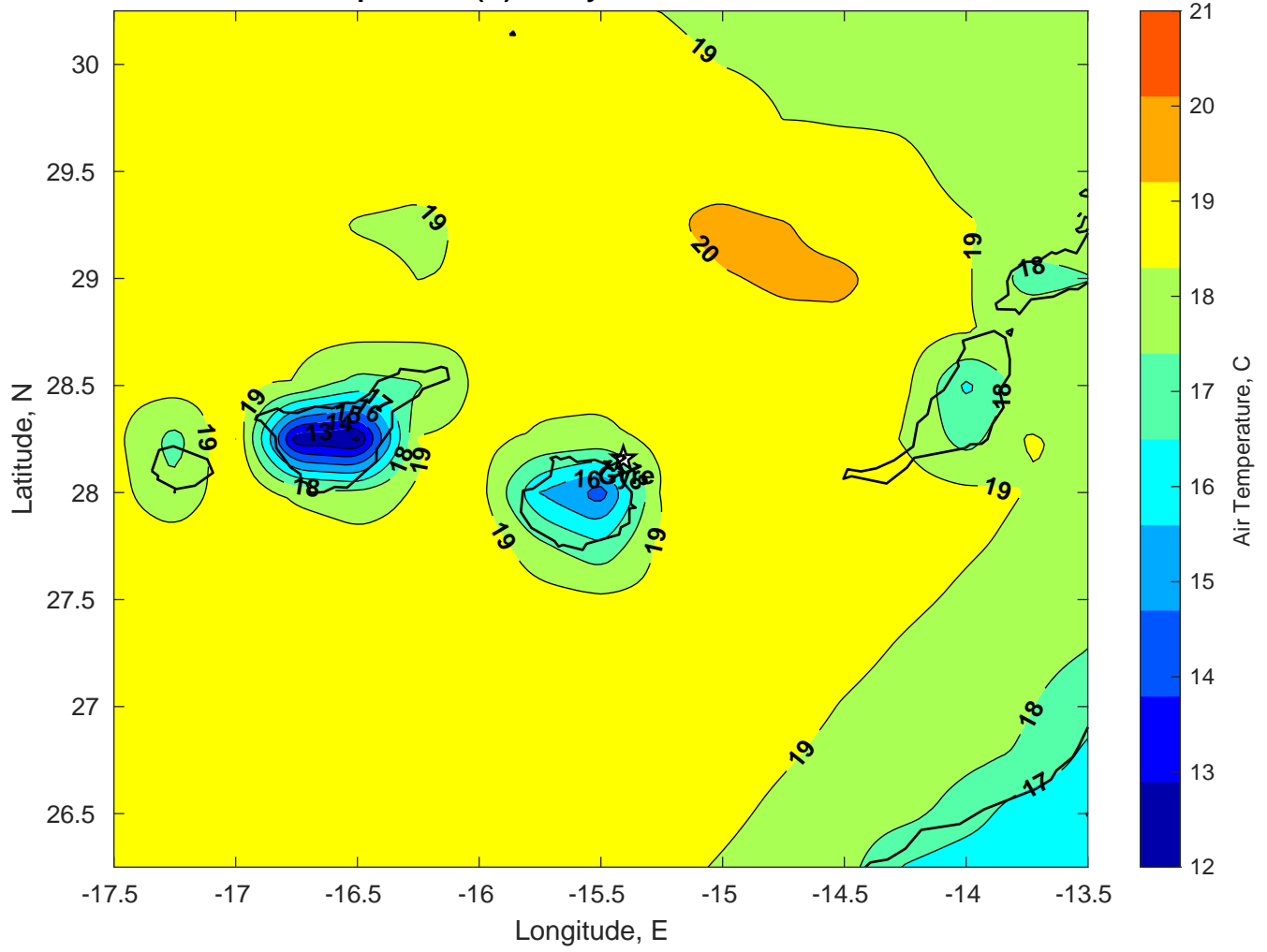
Air Temperature (C) for Gyre at 26-Feb-2025
