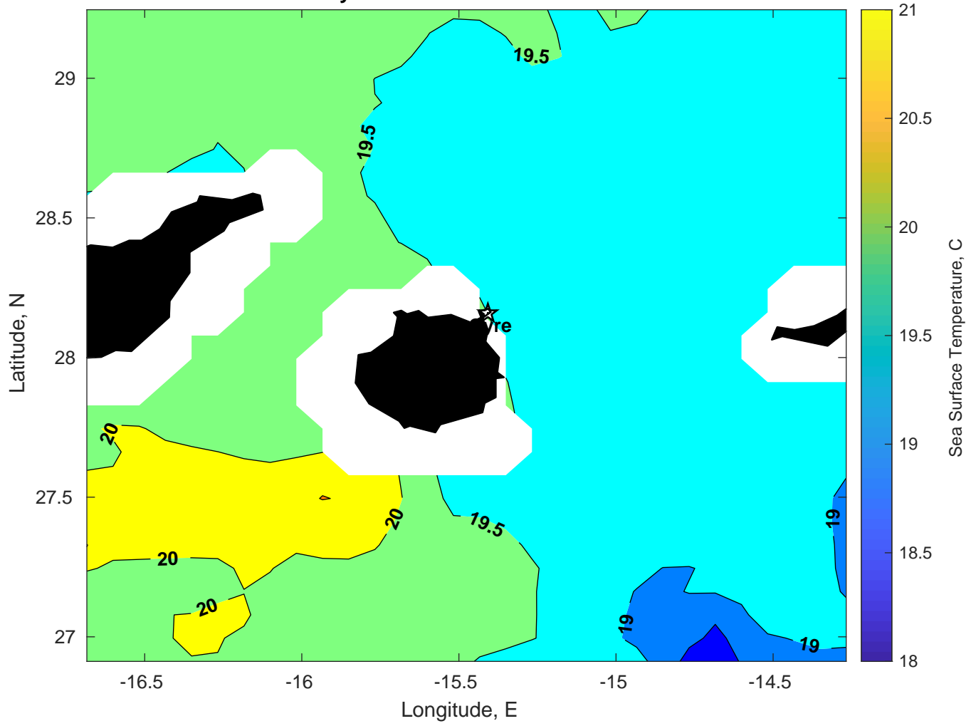
SST for Gyre at 25-Feb-2025 00:00:00
