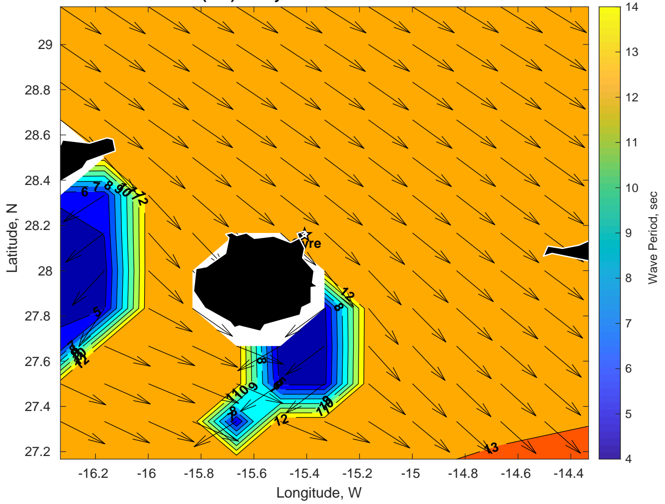
Wave Period (sec) for Gyre at 26-Feb-2025 09:00:00
