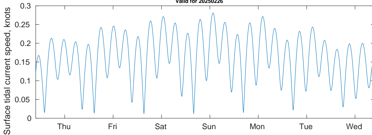
Tidal Currents and Heights for Gyre at 20250226
