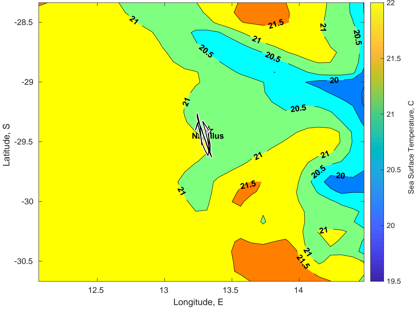
SST for Nautilus at 25-Feb-2025 00:00:00
