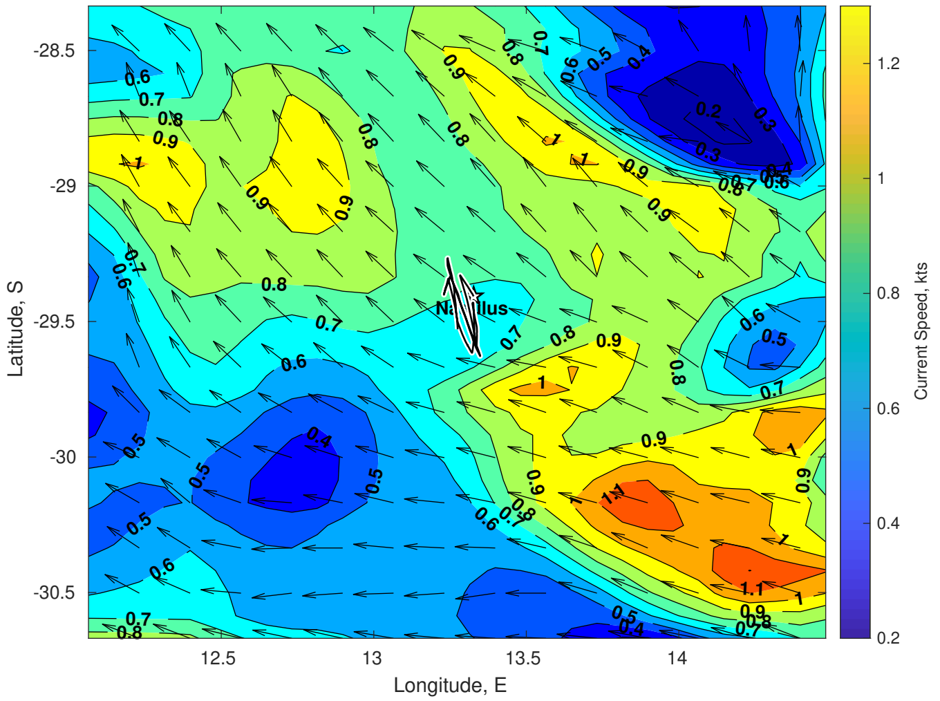
Surface Currents for Nautilus at 25-Feb-2025 00:00:00
