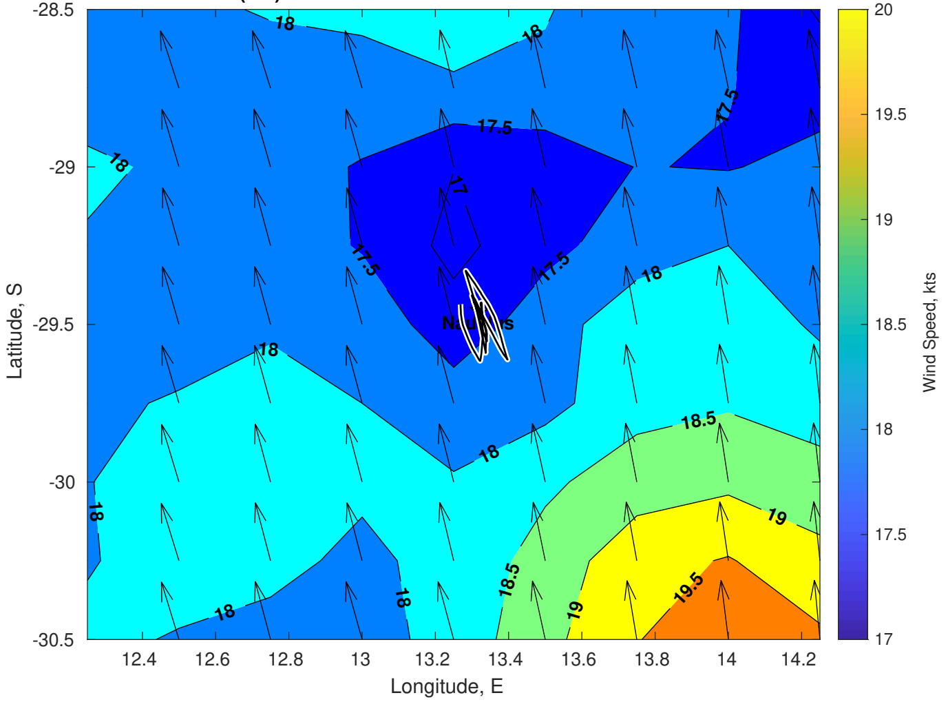
Winds (kts) for Nautilus at 26-Feb-2025 09:00:00
