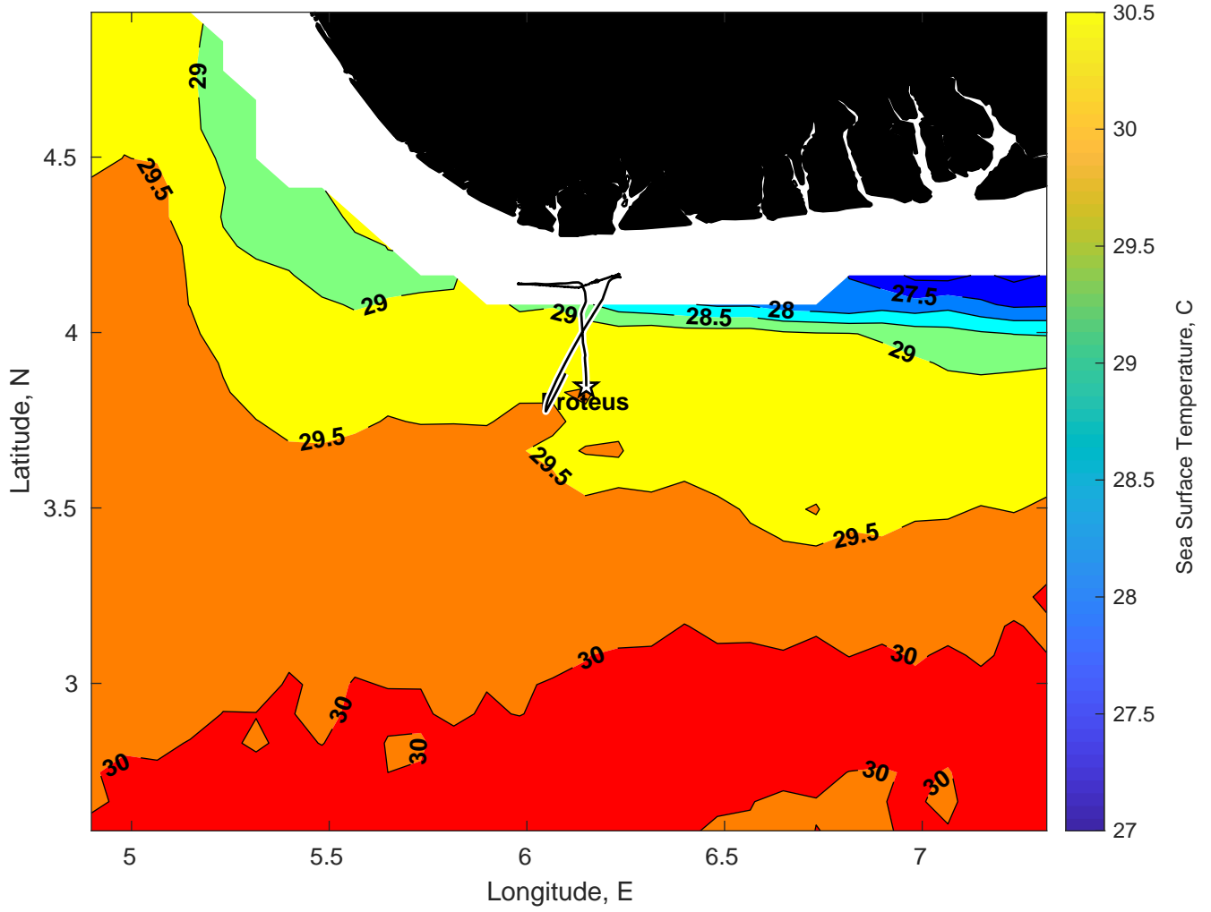
SST for Proteus at 25-Feb-2025 00:00:00
