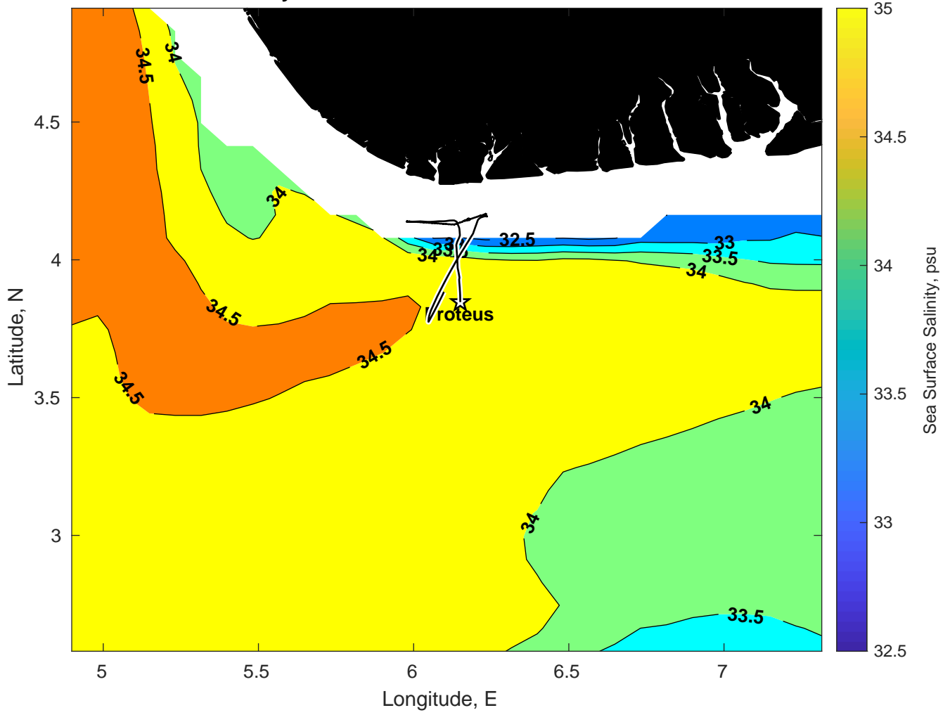
Surface Salinity for Proteus at 25-Feb-2025 00:00:00
