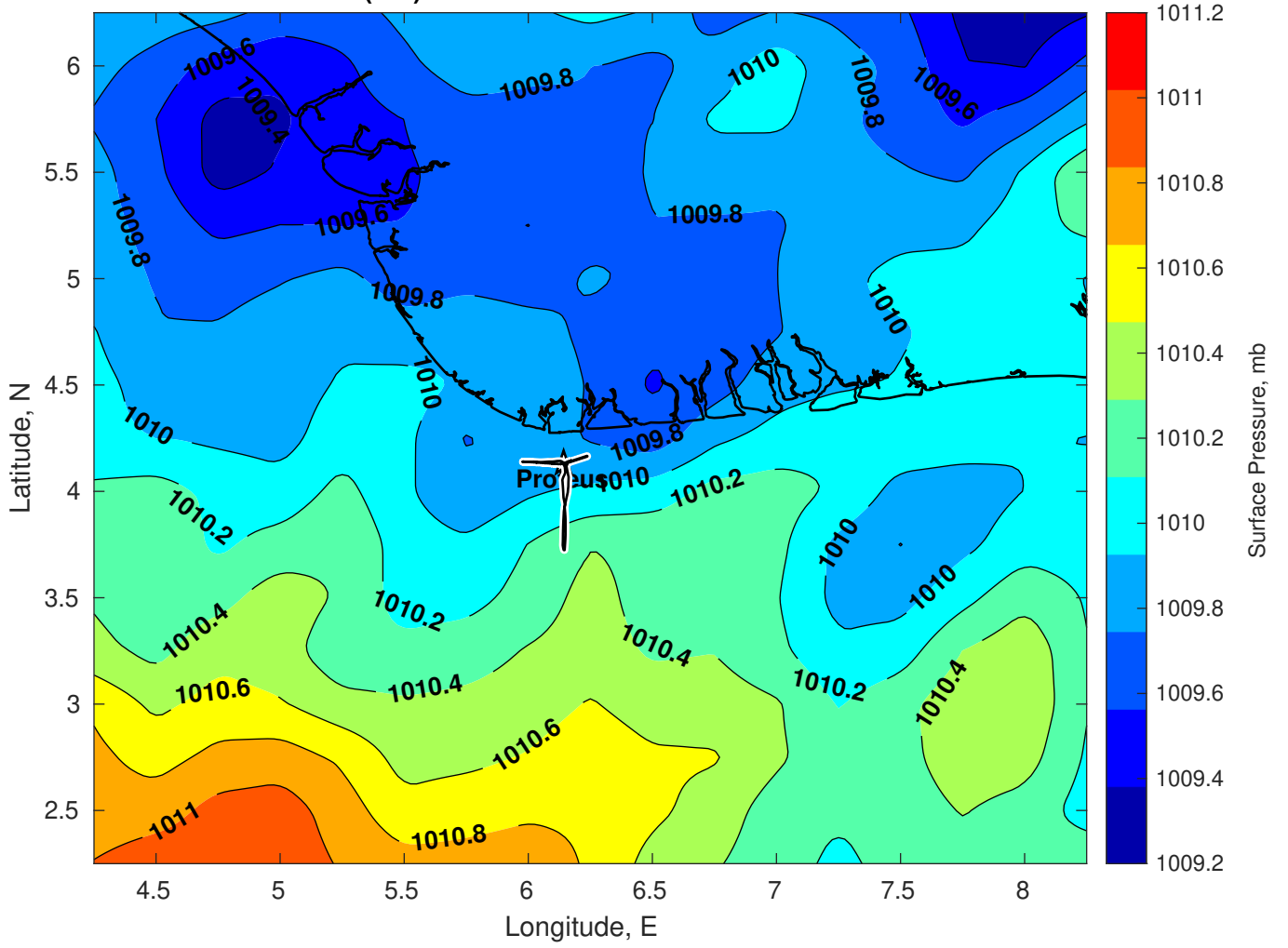
Surface Pressure (mb) for Proteus at 28-Feb-2025 00:00:00
