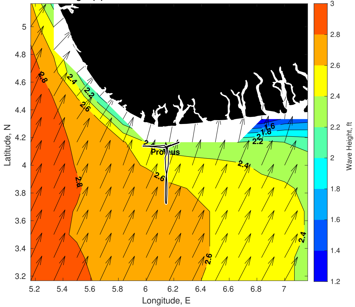
Wave Height (ft) for Proteus at 26-Feb-2025 09:00:00
