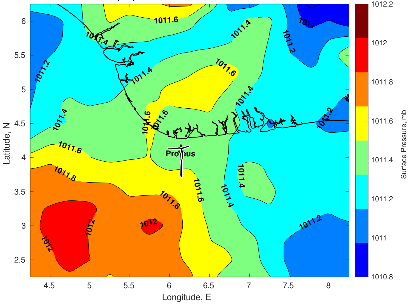
Surface Pressure (mb) for Proteus at 27-Feb-2025 00:00:00
