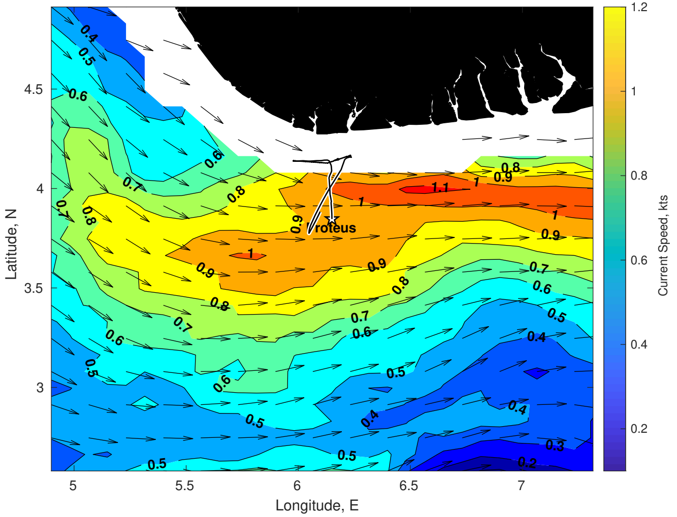
Surface Currents for Proteus at 25-Feb-2025 00:00:00
