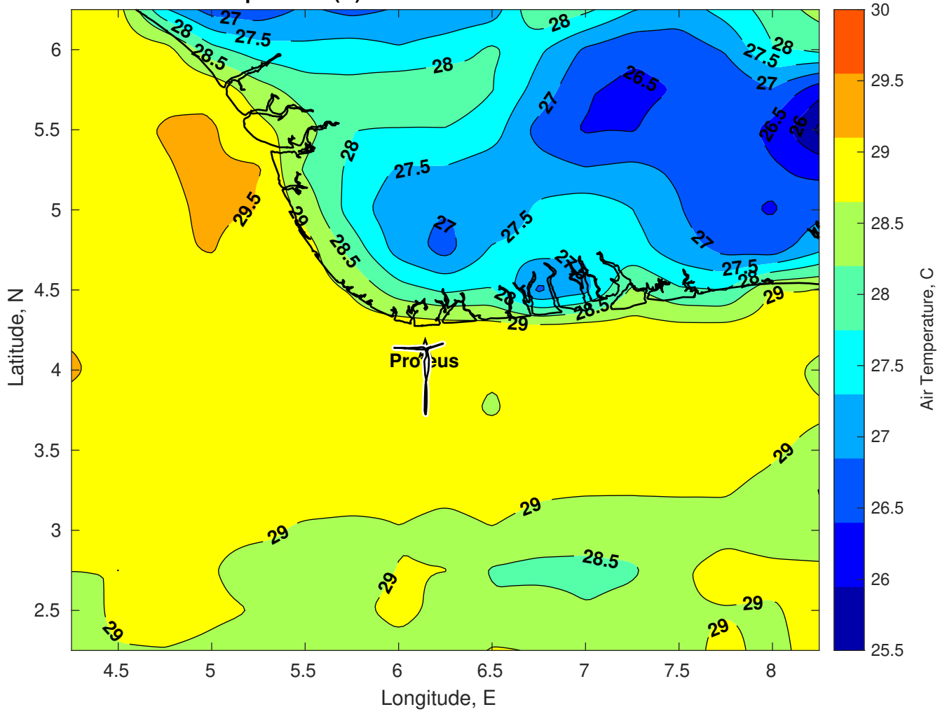
Air Temperature (C) for Proteus at 26-Feb-2025
