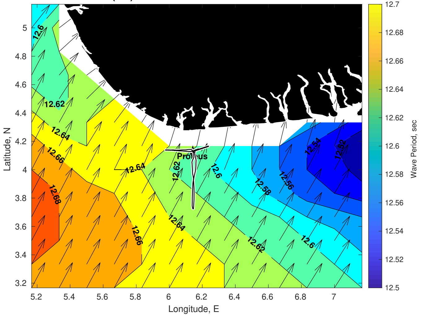
Wave Period (sec) for Proteus at 26-Feb-2025 09:00:00
