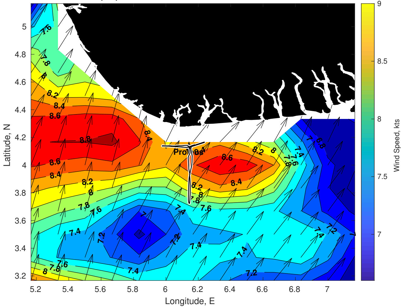
Winds (kts) for Proteus at 26-Feb-2025 09:00:00
