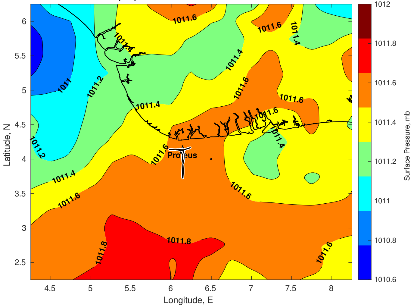
Surface Pressure (mb) for Proteus at 26-Feb-2025 00:00:00
