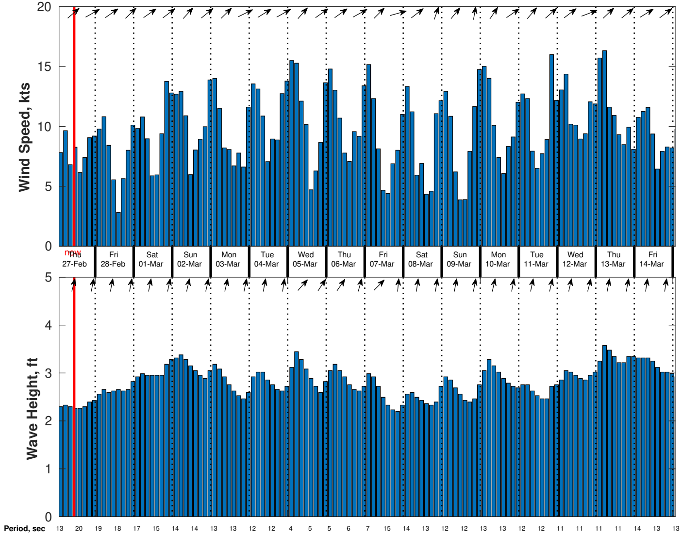
Wind & Wave Forecast for Proteus from 26-Feb-2025 01:00:00 to 14-Mar-2025 01:00:00
