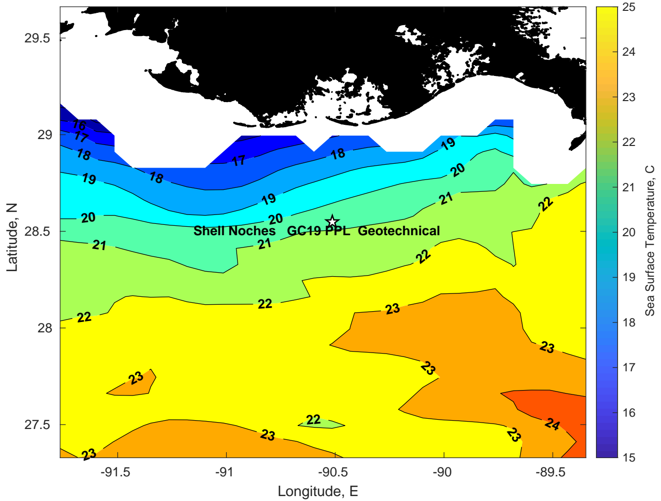
SST for Shell Noches GC19 PPL Geotechnical at 25-Feb-2025 00:00:00
