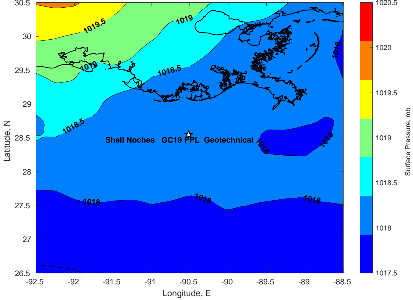
Surface Pressure (mb) for Shell Noches GC19 PPL Geotechnical at 28-Feb-2025 00:00:00
