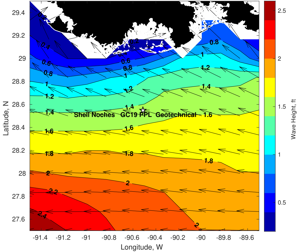
Wave Height (ft) for Shell Noches GC19 PPL Geotechnical at 26-Feb-2025 09:00:00
