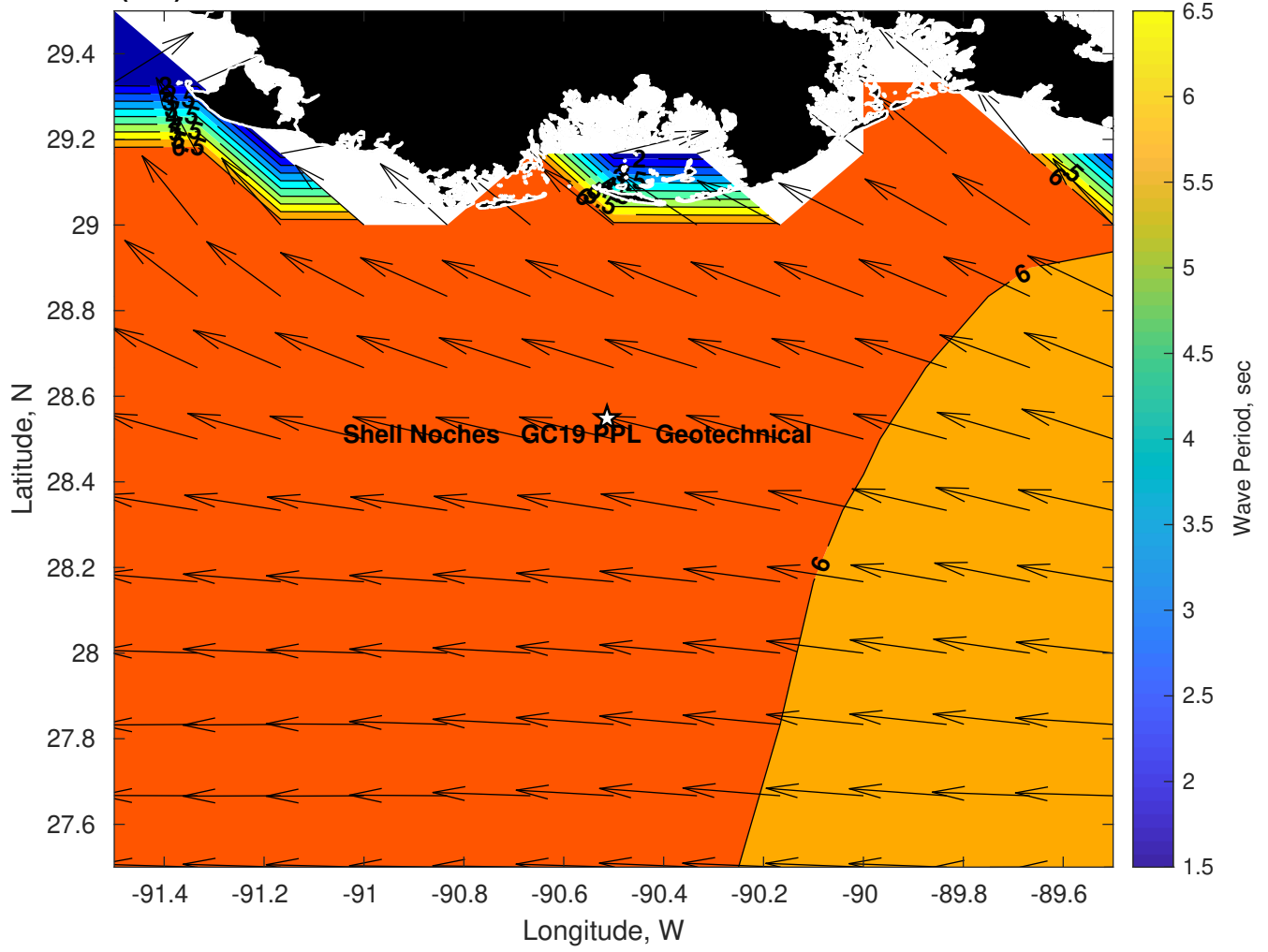
Wave Period (sec) for Shell Noches GC19 PPL Geotechnical at 26-Feb-2025 09:00:00
