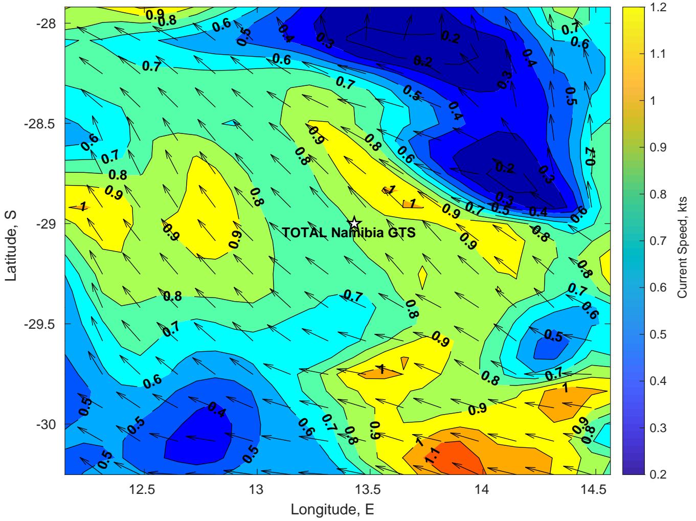
Surface Currents for TOTAL Namibia GTS at 25-Feb-2025 00:00:00
