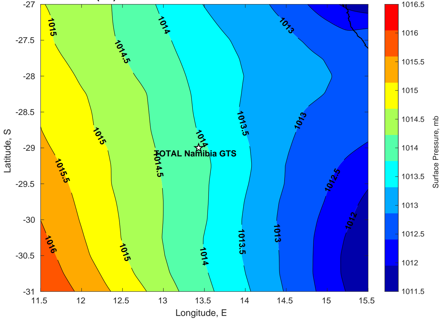
Surface Pressure (mb) for TOTAL Namibia GTS at 27-Feb-2025 00:00:00
