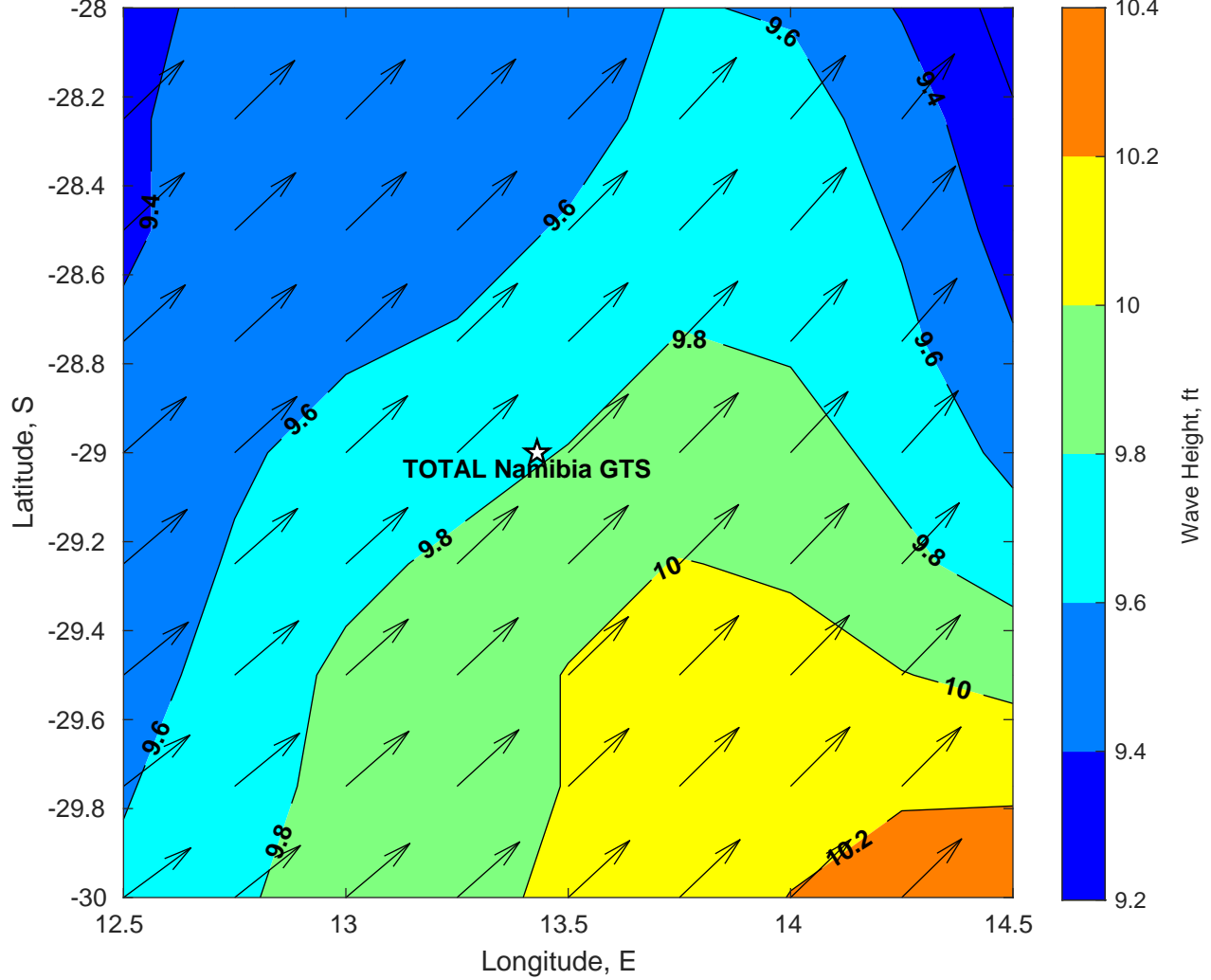
Wave Height (ft) for TOTAL Namibia GTS at 26-Feb-2025 09:00:00
