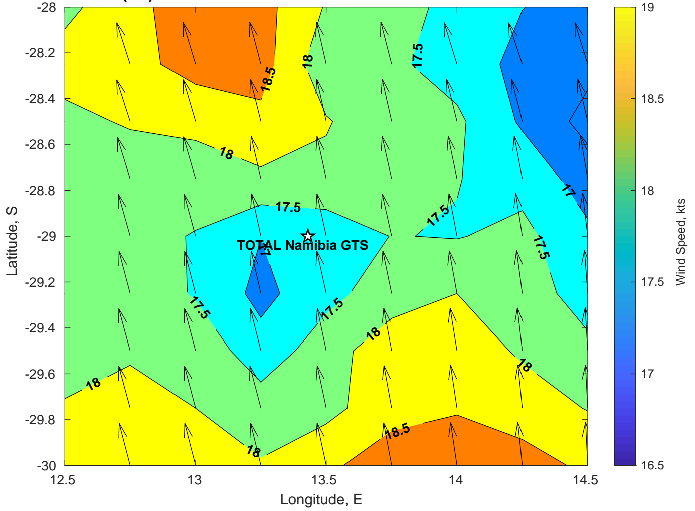
Winds (kts) for TOTAL Namibia GTS at 26-Feb-2025 09:00:00
