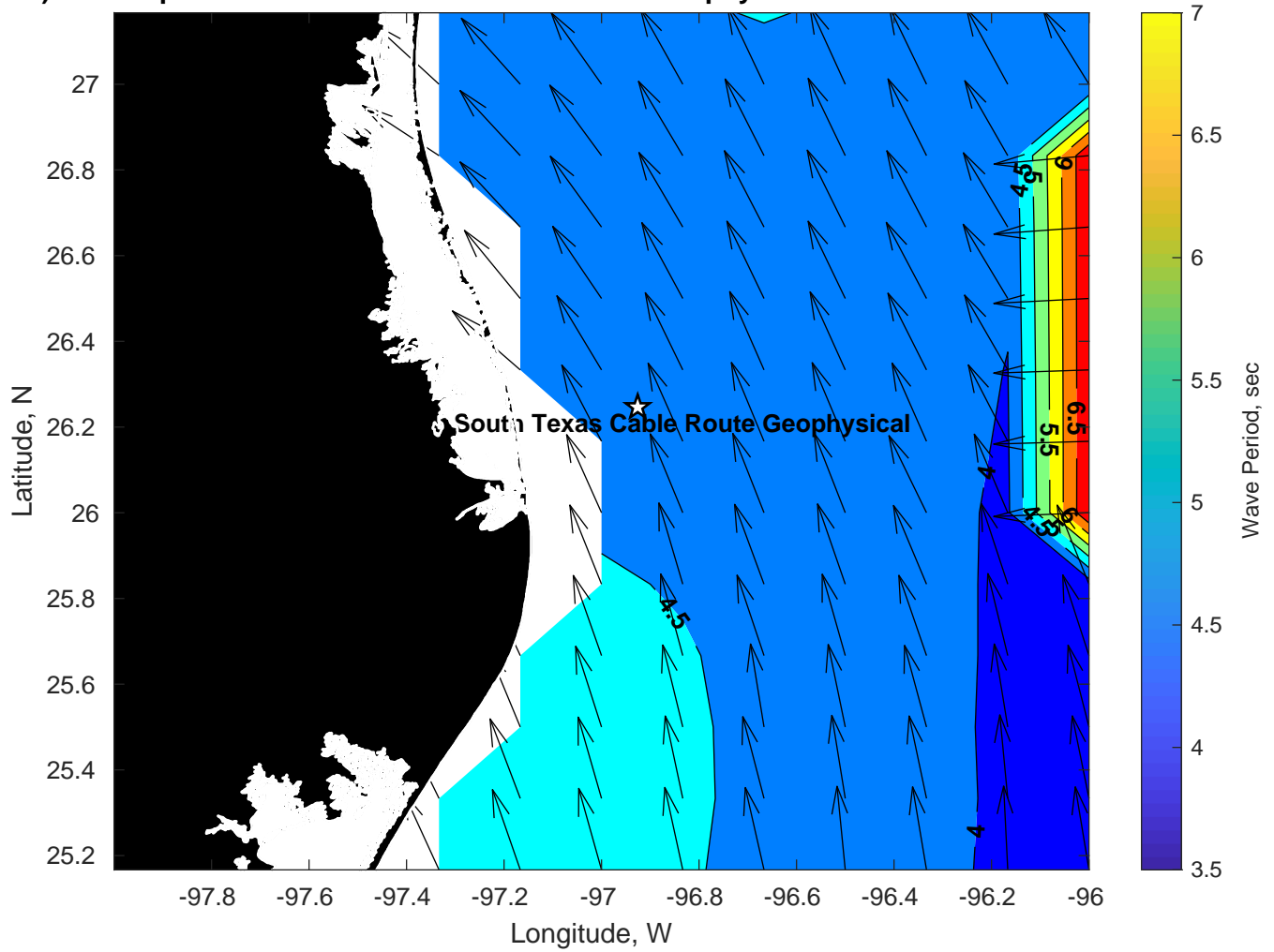
Period (sec) for Tampnet P2378 South Texas Cable Route Geophysical at 26-Feb-2025 09:00:00
