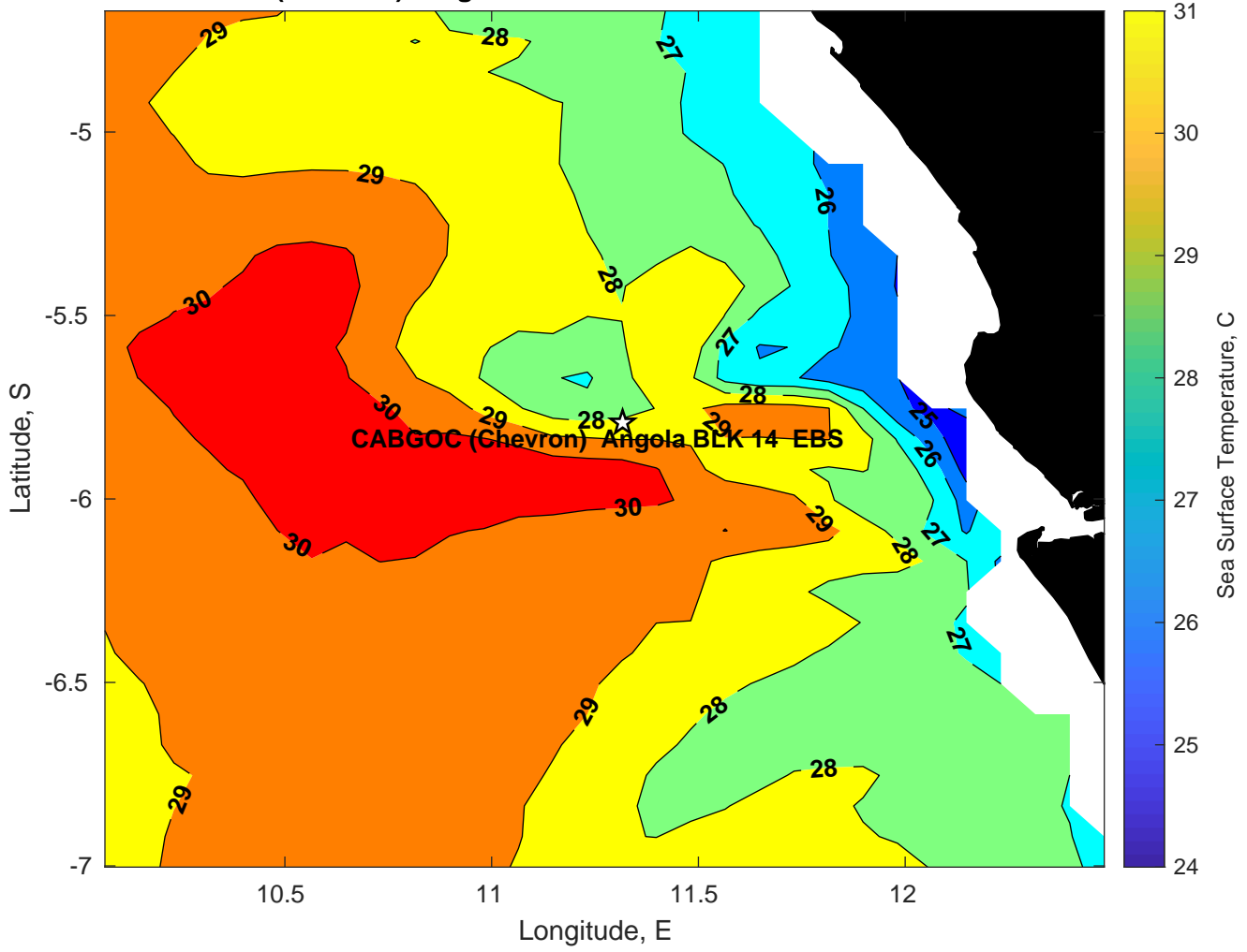
SST for CABGOC (Chevron) Angola BLK 14 EBS at 26-Feb-2025 00:00:00
