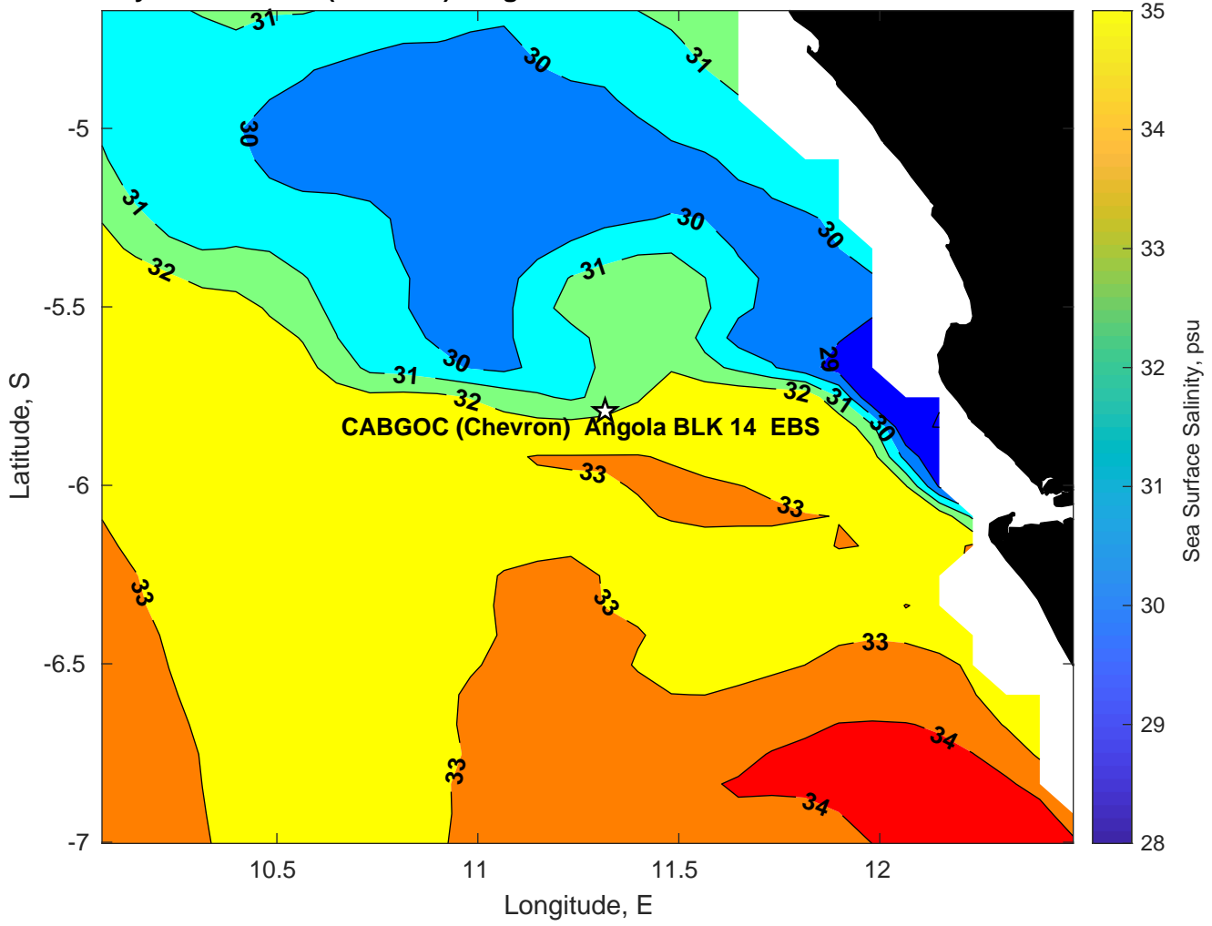
Surface Salinity for CABGOC (Chevron) Angola BLK 14 EBS at 26-Feb-2025 00:00:00
