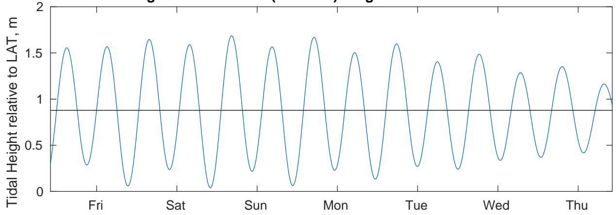
Tidal Currents and Heights for CABGOC (Chevron) Angola BLK 14 EBS at 20250227
