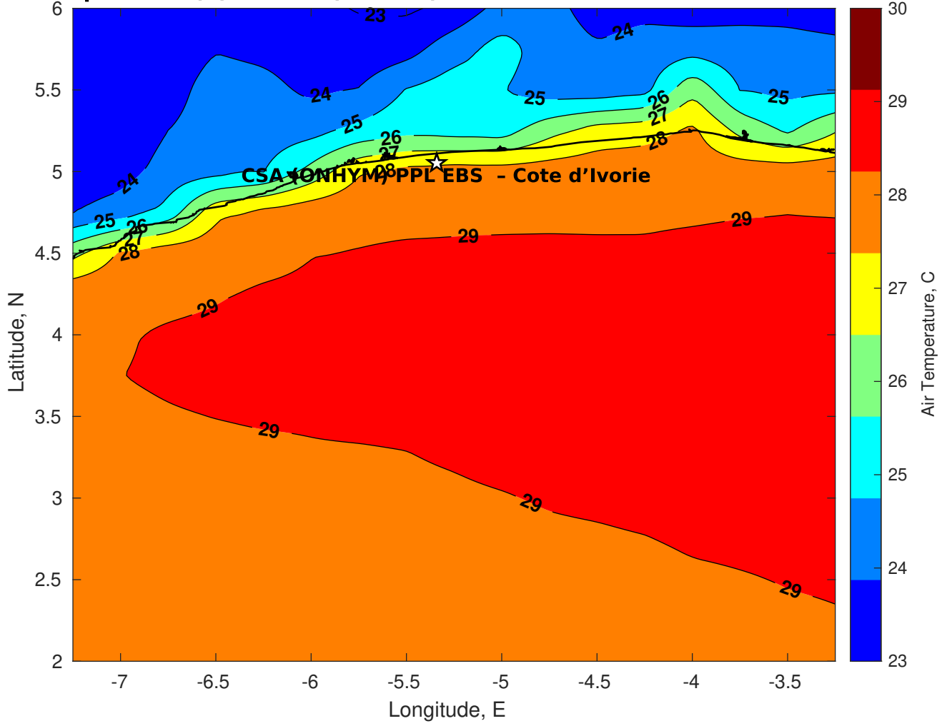
Air Temperature (C) for CSA (ONHYM) PPL EBS - Cote d'Ivoire at 27-Feb-2025
