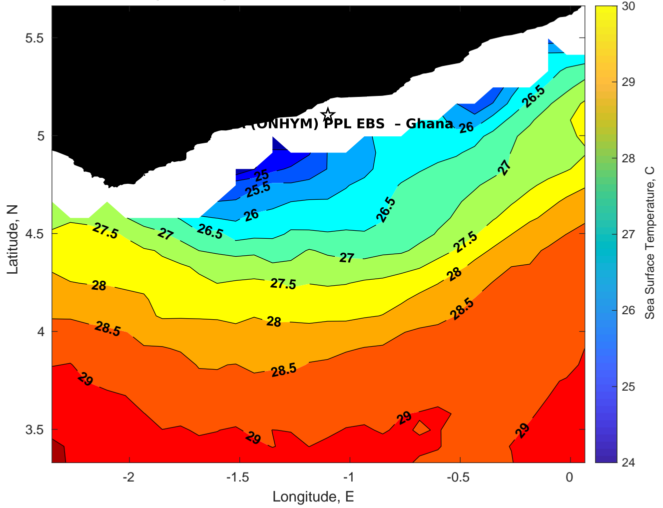
SST for CSA (ONHYM) PPL EBS - Ghana at 26-Feb-2025 00:00:00
