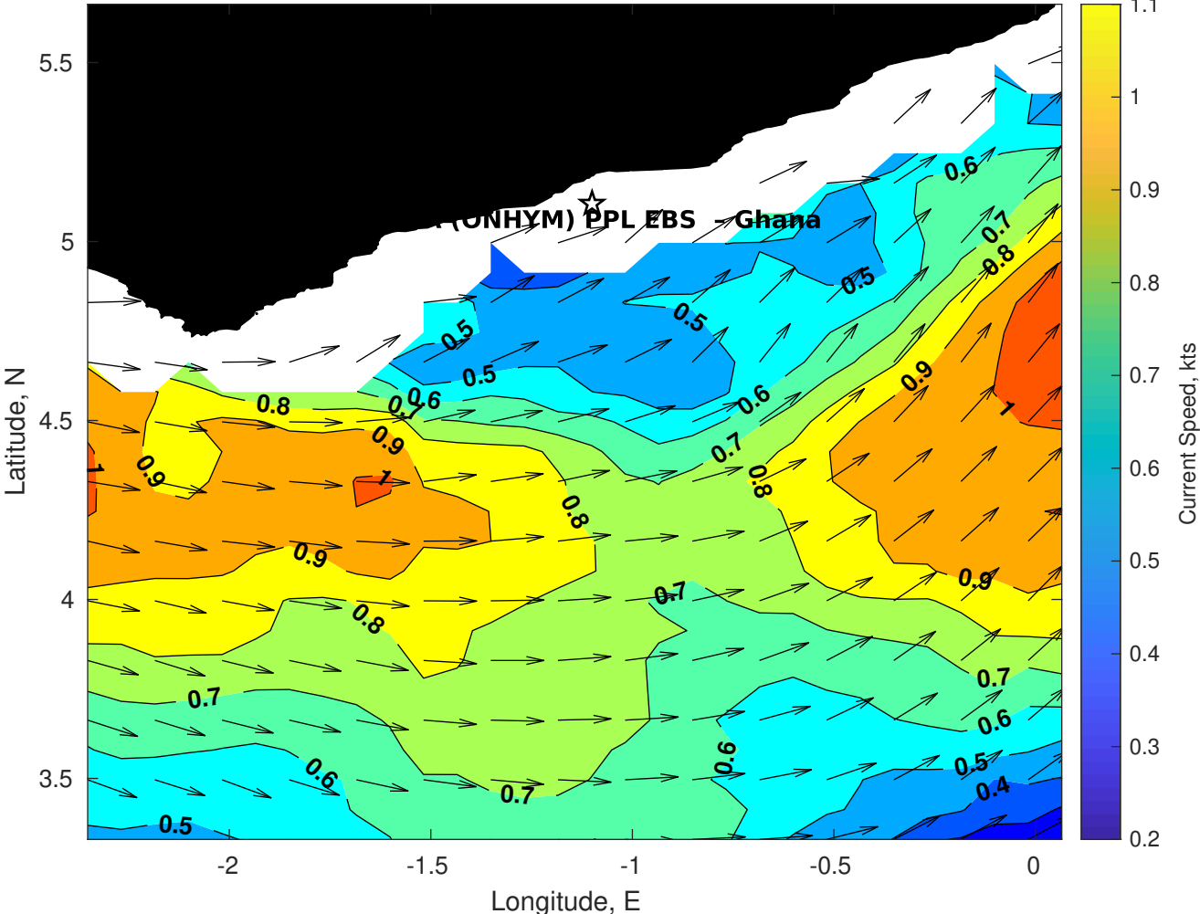
Surface Currents for CSA (ONHYM) PPL EBS - Ghana at 26-Feb-2025 00:00:00
