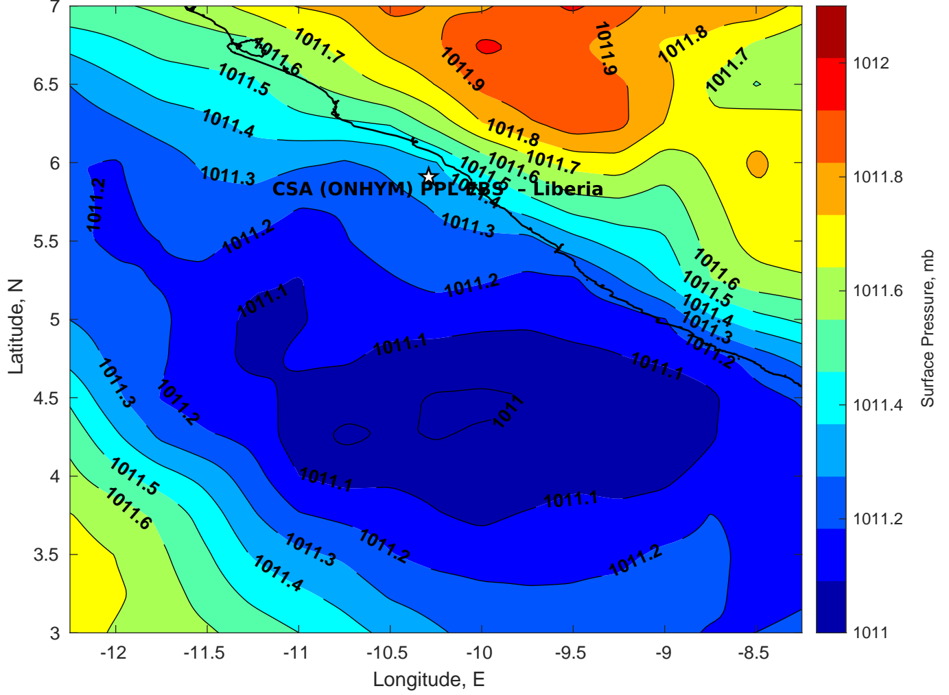
Surface Pressure (mb) for CSA (ONHYM) PPL EBS - Liberia at 28-Feb-2025 00:00:00
