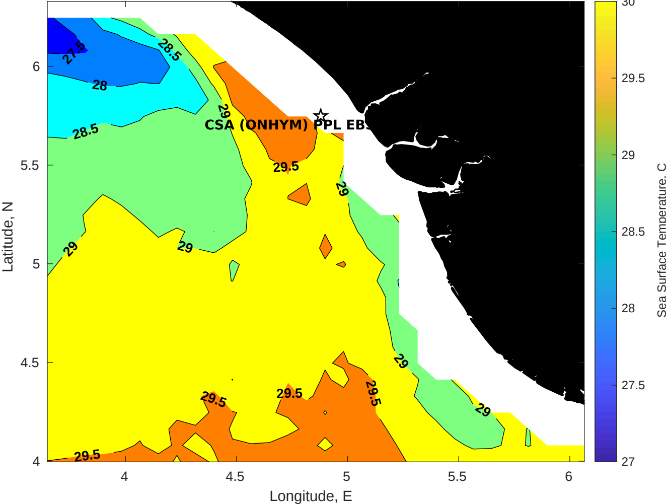
SST for CSA (ONHYM) PPL EBS - Nigeria at 26-Feb-2025 00:00:00
