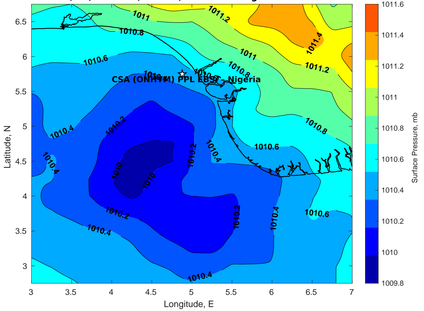
Surface Pressure (mb) for CSA (ONHYM) PPL EBS - Nigeria at 27-Feb-2025 06:00:00
