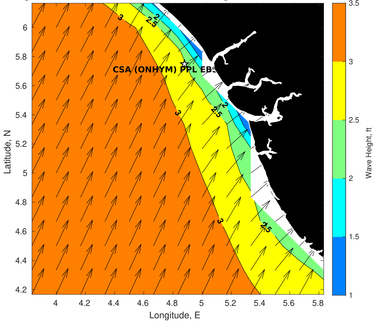
Wave Height (ft) for CSA (ONHYM) PPL EBS - Nigeria at 27-Feb-2025 09:00:00
