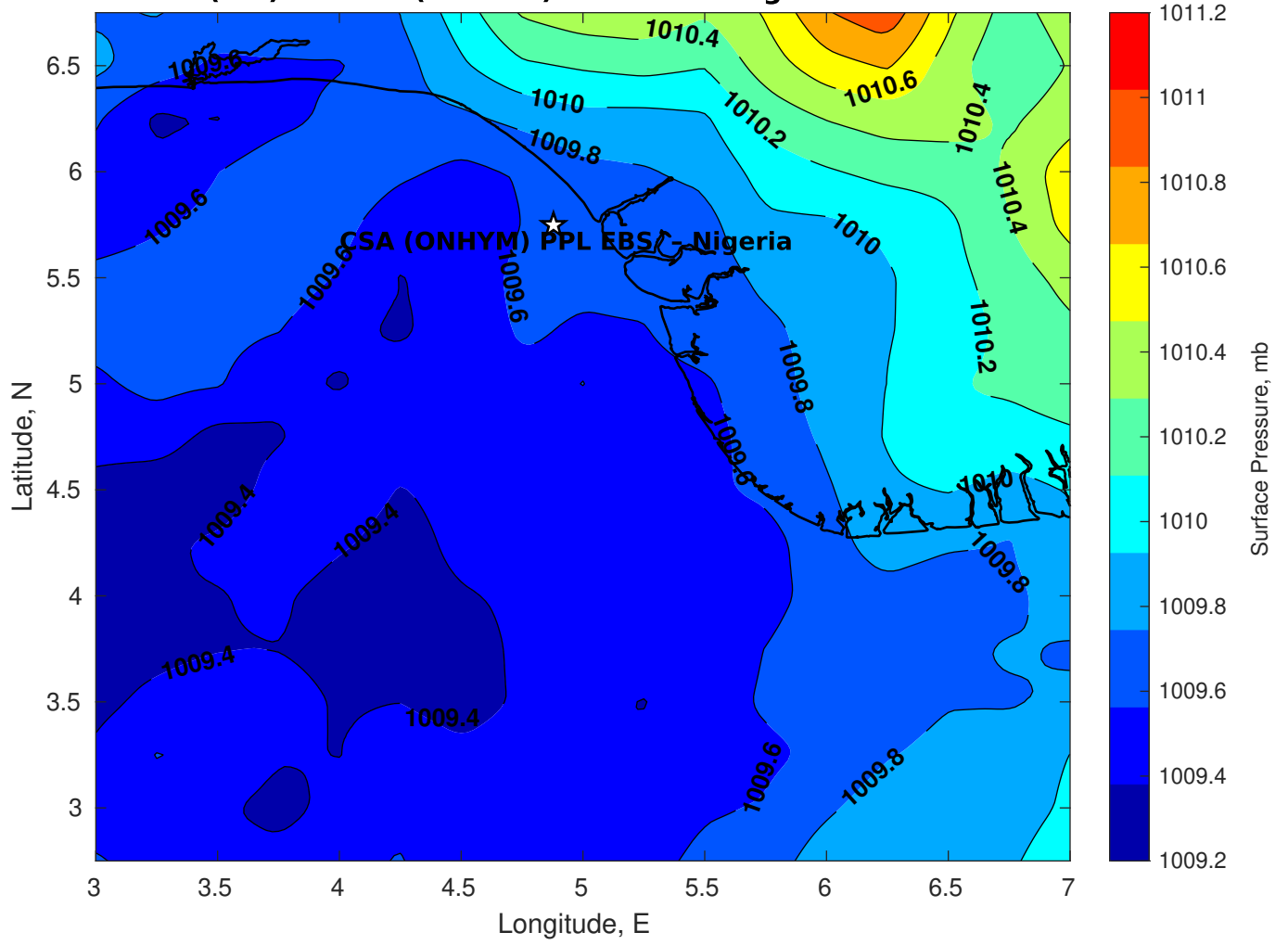
Surface Pressure (mb) for CSA (ONHYM) PPL EBS - Nigeria at 28-Feb-2025 06:00:00
