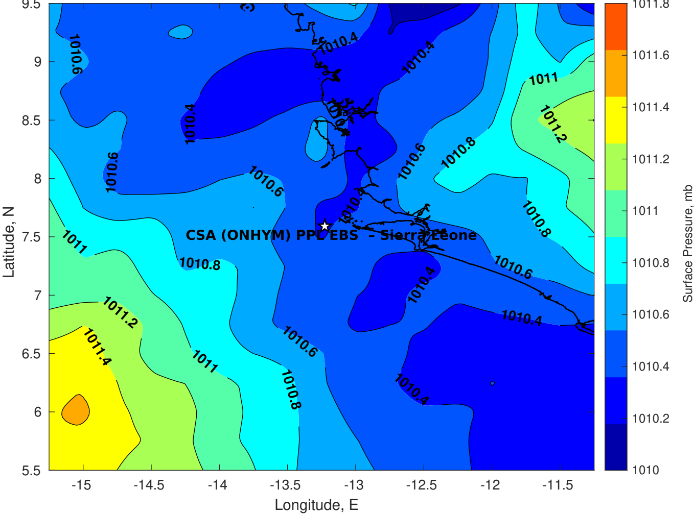
Surface Pressure (mb) for CSA (ONHYM) PPL EBS - Sierra Leone at 01-Mar-2025 00:00:00
