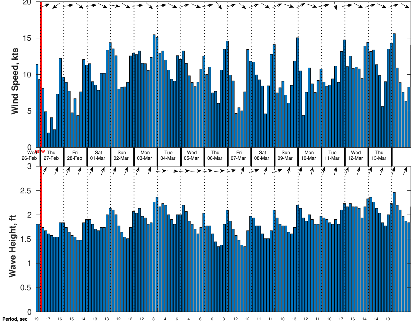
Wind & Wave Forecast for CSA (ONHYM) PPL EBS - Sierra Leone from 26-Feb-2025 19:00:00 to 14-Mar-2025 19:00:00
