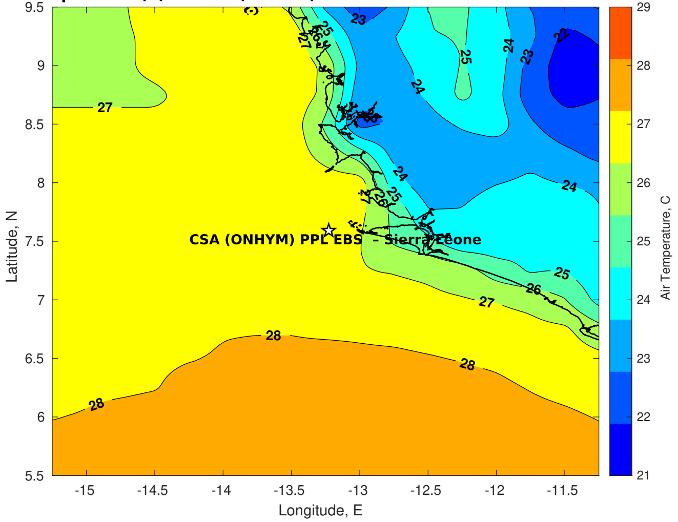
Air Temperature (C) for CSA (ONHYM) PPL EBS - Sierra Leone at 27-Feb-2025
