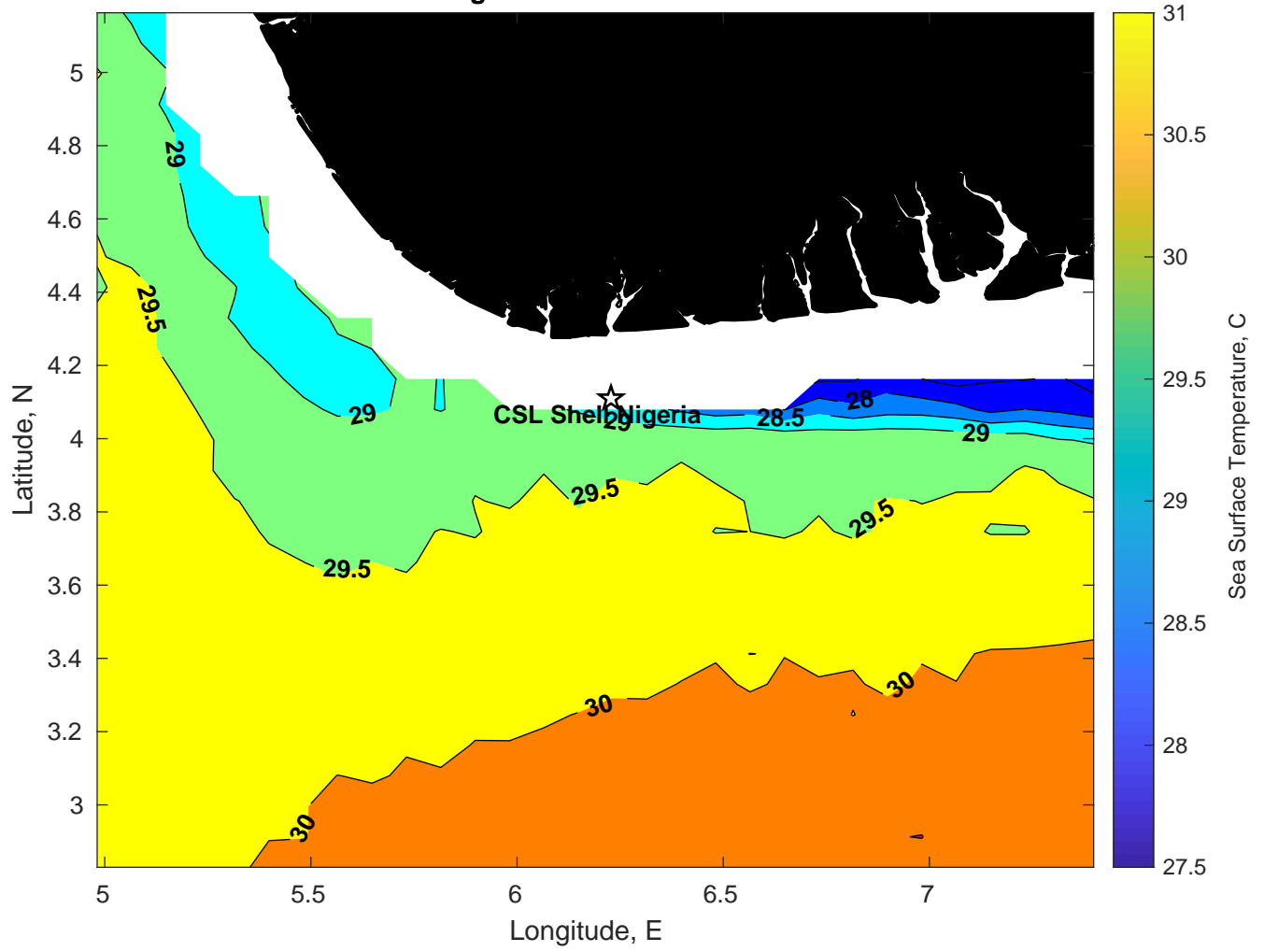
SST for CSL Shell Nigeria at 26-Feb-2025 00:00:00
