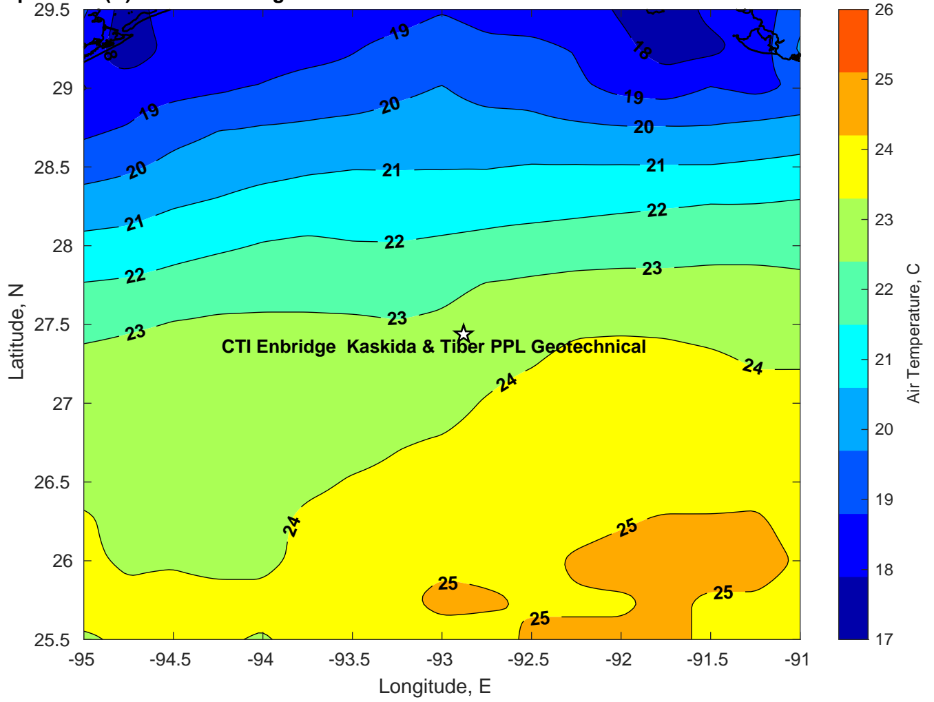
Air Temperature (C) for CTI Enbridge Kaskida & Tiber PPL Geotechnical at 27-Feb-2025
